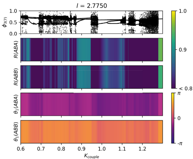
Fig. 5. \phi_{3(7)} Value which \phi_3 assumes on the Poincaré section in which we save values at each 7 days, abbreviation in figure R(\phi_{3AB(l)}, \phi_{3A}) as R(ABA) , R(\phi_{3AB(l)}, \phi_{3B}) as R(ABB) , \theta_1(\phi_{3AB(l)}, \phi_{3A}) as \theta_1(ABA) and \theta_1(\phi_{3AB(l)}, \phi_{3B}) as \theta_1(ABB) .
