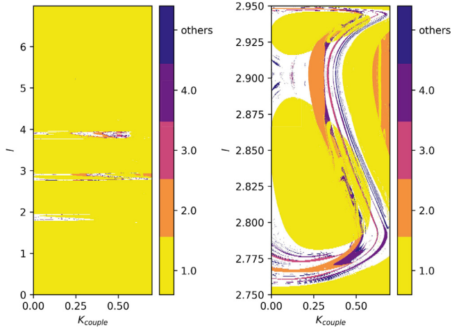
Fig. 6. Parameter space of the period. The white regions are the regions that the algorithm could not find a period, either because it is too high or because the solution is chaotic. The other periods are indicated in the legend next to the panels.
