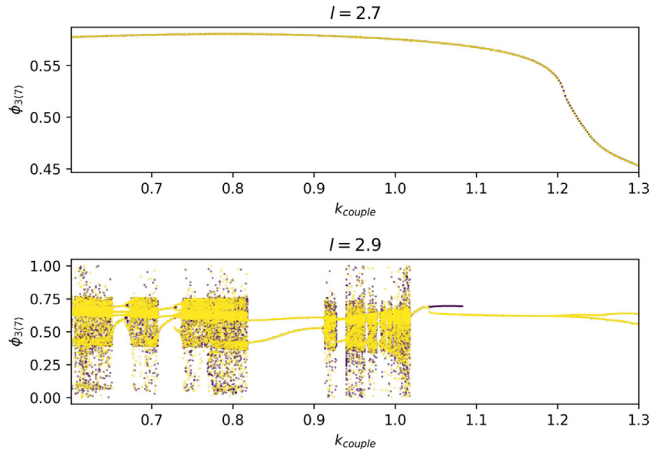
Fig. 7. Value that \phi_3 assumes on the Poincaré section in which we take values at each seven days, for l = 2.7 and l = 2.9 following the attractor. In yellow (lighter gray on the impressed version) simulations with K_{couple} increasing and in purple (darker gray on the impressed version) decreasing.
