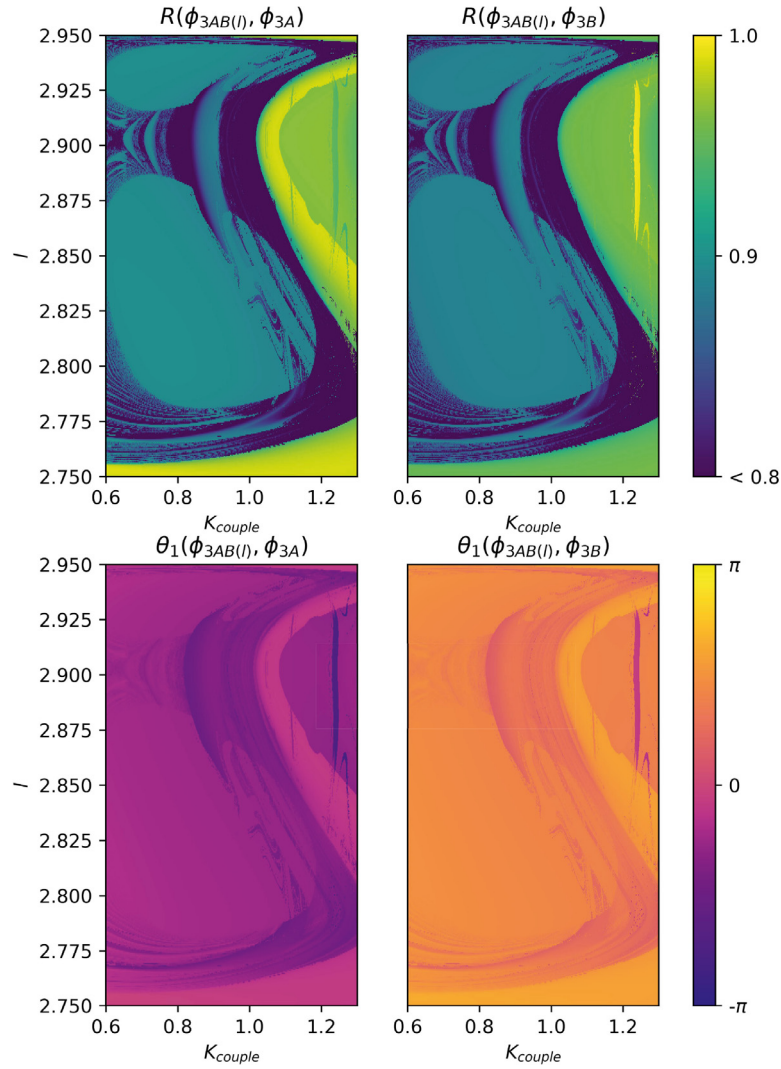
Fig. 4. Zoom of parameter spaces related to synchronization.
