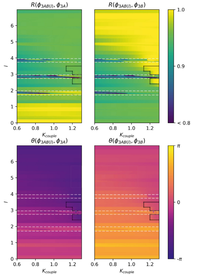
Fig. 3. Parameter spaces related to synchronization between \phi_{3AB(l)} and \phi_{3A} or \phi_{3B} , which are, respectively, the phases of oscillator 3 when the light input is AB(l) , A , and B . R(\phi_{3AB(l)}, \phi_{3A}) [ R(\phi_{3AB(l)}, \phi_{3B}) ] is a synchronization measurement between \phi_{3AB(l)} and \phi_{3A} [ \phi_{3B} ]. \theta(\phi_{3AB(l)}, \phi_{3A}) [ \theta(\phi_{3AB(l)}, \phi_{3B}) ] is the mean angle between \phi_{3AB(l)} and \phi_{3A} [ \phi_{3B} ]. K_{couple} is the control parameter, l[7-l] is the number of days in the week that correspond to light input B[A] in the light input AB(l) .
