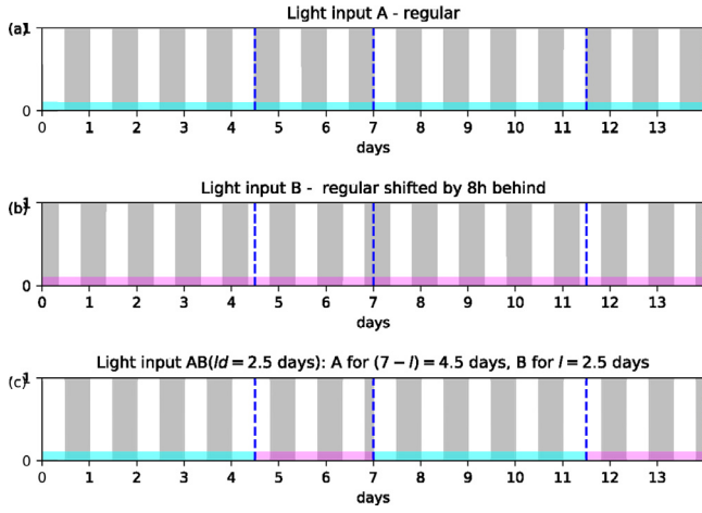
Fig. 1. (a) Light input A - regular light input, 12 h of light (–12 to 0) followed by 12 h of dark (0 to 12). (b) Light input B 12 h of light (–4 to 8) followed by 12 h of dark (8 to –4), in other words, light input A with a delay of 8 h (c) Light input AB( l = 2.5 ), light input A for 4.5 days followed by light input B for 2.5 days.
