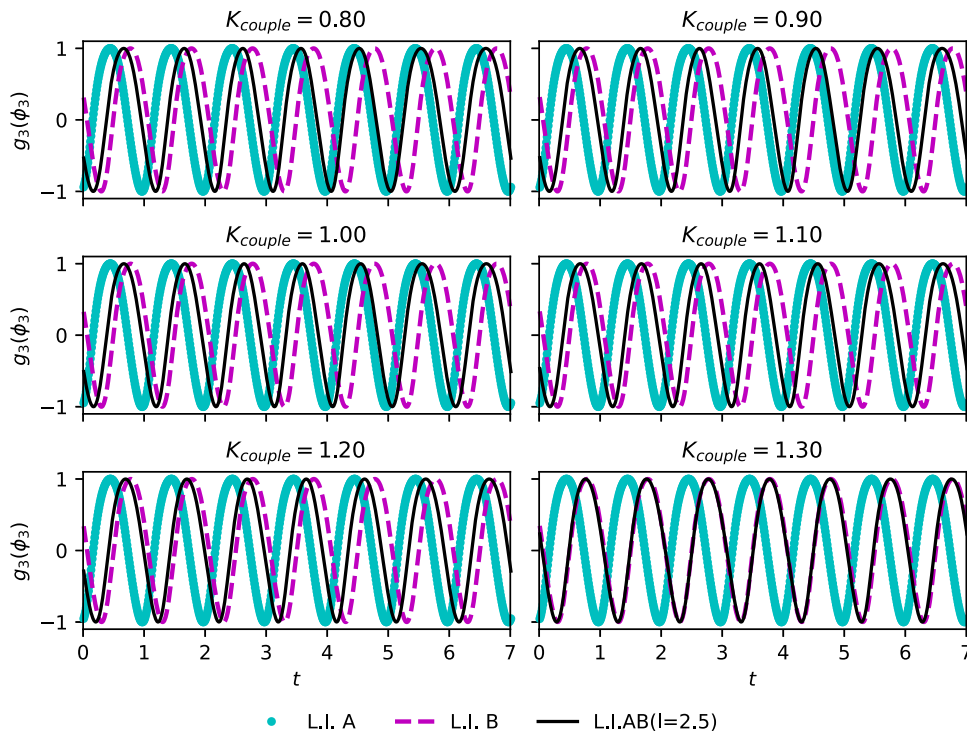
Fig. 2. The dotted cyan line corresponds to the output g_3(\phi_3) for the light input A, the dashed pink line for the light input B and the black continuous line for the light input AB( l = 2.5 ). In each panel the value of the coupling parameter K_{couple} is indicated.
