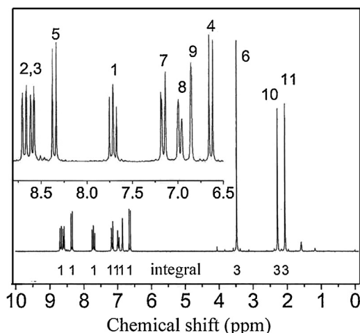
Fig. 2. NPOX nuclear magnetic resonance of proton ( ^1\text{H} NMR) spectrum with \text{CHCl}_3 as solvent and tetramethylsilane as internal reference.
