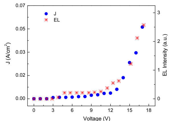
Fig. 9. EL intensity and current density of a ITO/PEDOT:PSS-(60 nm)/NPOX(100 nm)/Al(120 nm) OLED device as a function of applied voltage with ITO positively biased.
