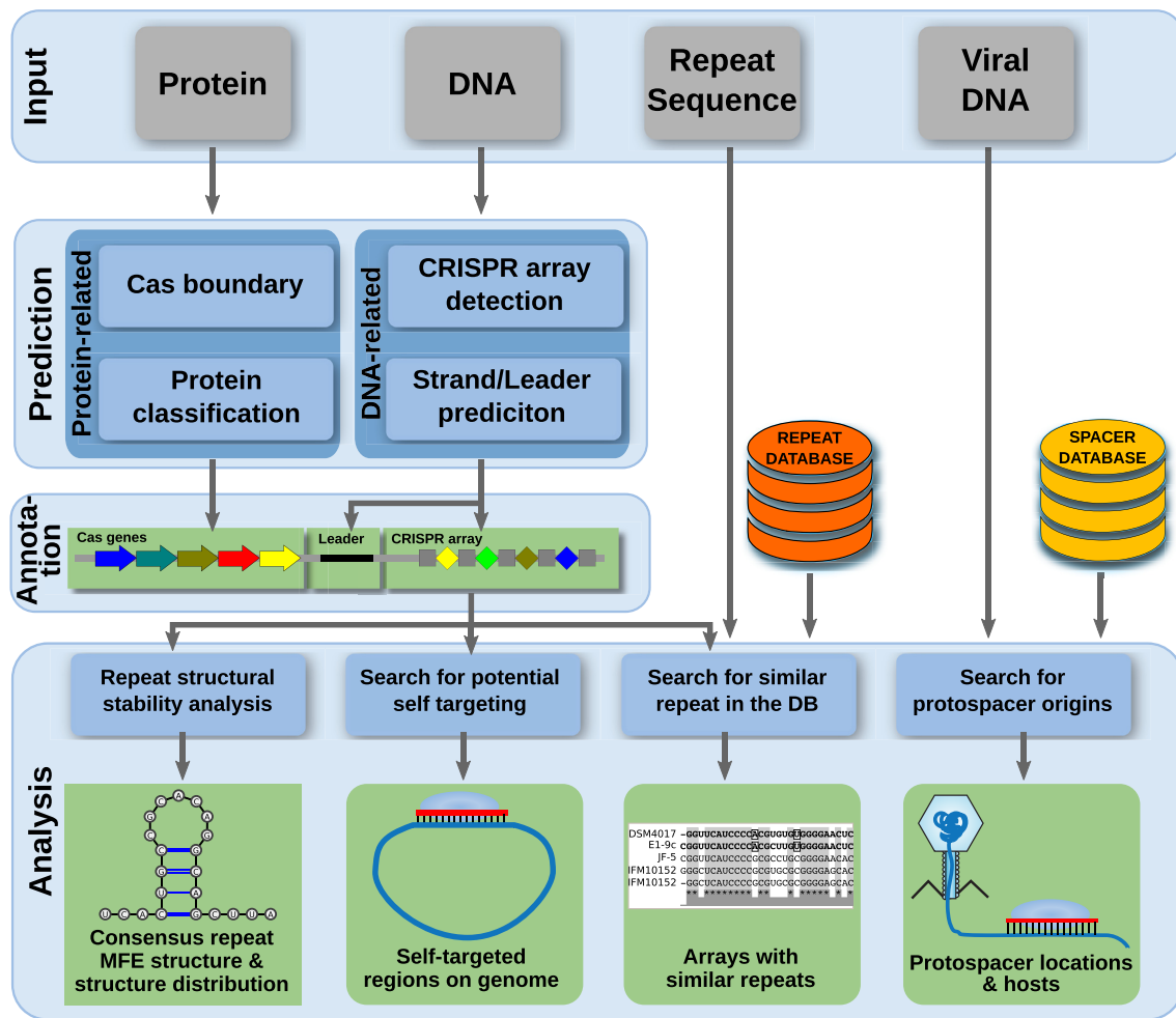
Figure 1. The workflow of CRISPRloci. The workflow supports 4 different types of input. If DNA is picked as the input, CRISPRloci will identify the CRISPR arrays , predict their orientation and the Leader sequence and then extract the repeat and spacer sequences. Repeat sequences are then analyzed for their structural stability while spacers are used to identify the potential regions of self targeting. If protein sequences are submitted as input, CRISPRloci will classify and report the protein type and role. The user can optionally input a set of repeat sequences. In this scenario, CRISPRloci will perform a search of similar repeat sequences in the existing database. The user will be provided with the hits as well as their region, similarity and e-value. Lastly, the user can provide viral DNA as the input. In this scenario, CRISPRloci will perform a search for the protospacers using a database of spacers. The user will be provided with the protospacer coordinates as well as the description of the host CRISPR arrays .
