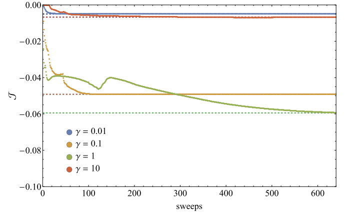
Fig. 9. Spin current convergence versus sweep number for different coupling values \gamma . Values used: N = 25 , \Delta = 1 , f_1 = 1 , f_N = 0 , h = 0 . Dashed lines correspond to the analytical solutions in [3].
