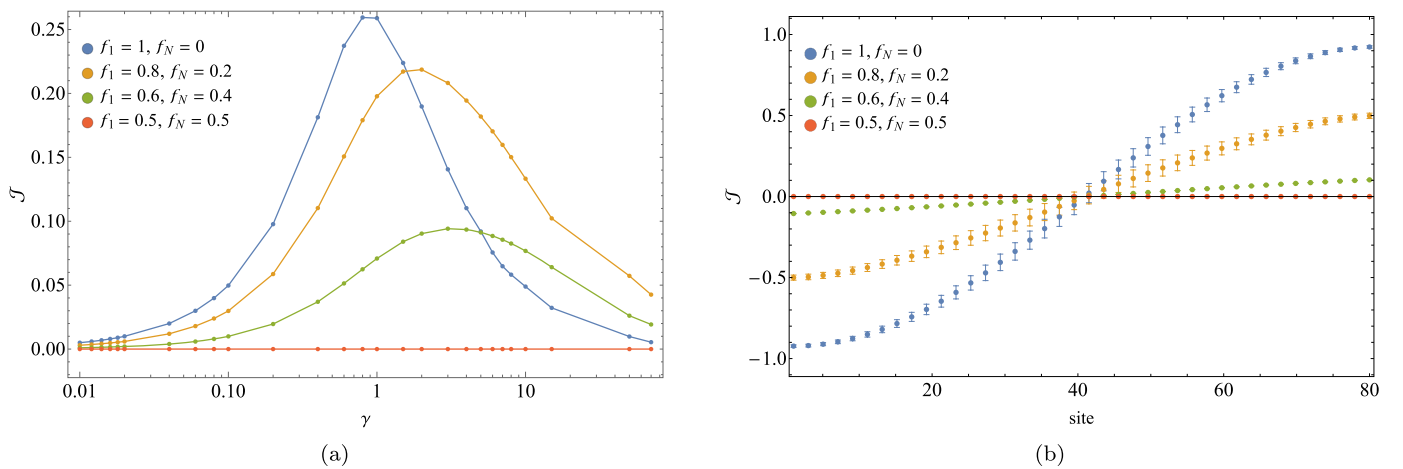
Fig. 12. (a) \mathcal{J} vs. \gamma for N = 10 and different values of f_1 , f_N . (b) Magnetization profile for N = 80 . Other parameters were \gamma = 0.5 , \Delta = 1 , h = 0 .
