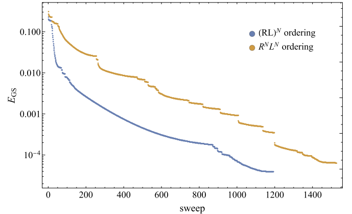
Fig. 6. Energy as a function of the number of sweeps, for the (RL)^N and R^N L^N orderings, with a fixed maximum bond dimension of 100. Values used: N = 20 , \gamma = 1 , \Delta = 0.5 , f_1 = 0.8 , f_N = 0.2 , h = 0 . (For interpretation of the colors in the figure(s), the reader is referred to the web version of this article.)
