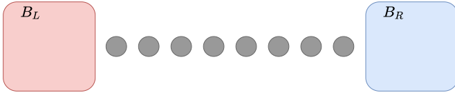
Fig. 1. Diagrammatic representation of a one-dimensional quantum spin chain coupled to two thermal baths B_L and B_R , one at each end. Here, each grey circle represent a spin.
