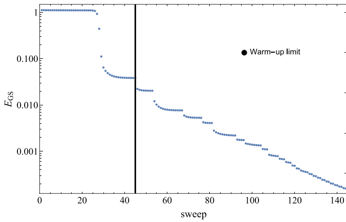
(a) Ground-state energy guess after each DMRG sweep
