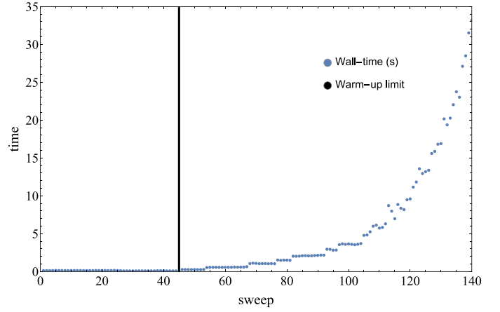
(b) Wall-time for each sweep
