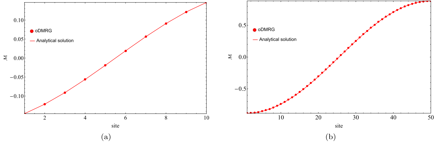
Fig. 11. Magnetization profile \mathcal{M} = \langle \sigma_z^i \rangle as a function of the sites for \gamma = 0.5 , for (a) N = 10 and (b) N = 50 . The red curves are the exact solutions from [3]. Other parameters were \Delta = 1 , f_1 = 1 , f_N = 0 , h = 0 .
