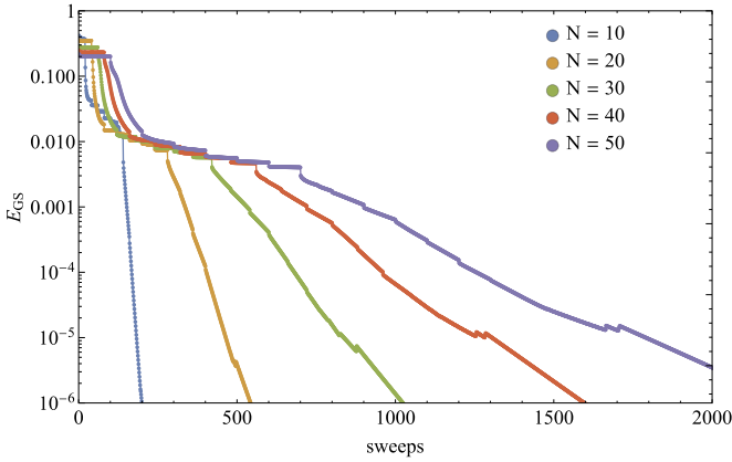
Fig. 8. Energy convergence for different chain lengths, after each sweep, for different system sizes N . Values used: \gamma = 1 , \Delta = 0.5 , f_1 = 1 , f_N = 0 , h = 0 .
