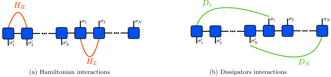
Fig. 4. Diagrammatic depiction of the Hamiltonian and dissipative terms under the R^N L^N formalism.
