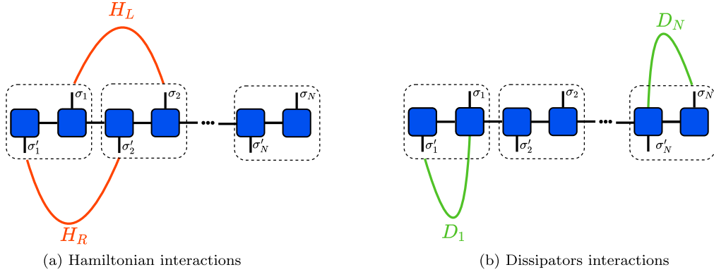
Fig. 5. Diagrammatic depiction of the Hamiltonian and dissipative terms under the (RL)^N formalism.
