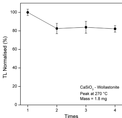
Fig. 6. Reproducibility of TL response of undoped \text{CaSiO}_3 synthetic irradiated with 1 Gy of ^{60}\text{Co} .
