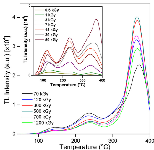
Fig. 9. TL glow curves of \text{CaSiO}_3:\text{Eu} (1000 ppm) irradiated with gamma dose of 0.5–1200 kGy.
