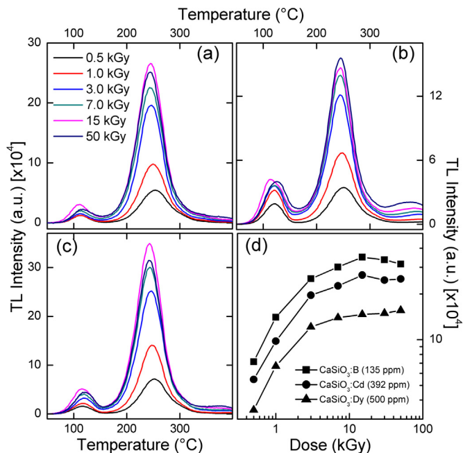
Fig. 8. TL glow curves of \text{CaSiO}_3:\text{x} (a) \text{x} = \text{Cd} , (b) \text{x} = \text{Dy} and (c) \text{x} = \text{B} irradiated with gamma dose of 0.5–50 kGy. (d) TL intensity versus doses of the TL peaks at 270^\circ\text{C} for three doped samples.
