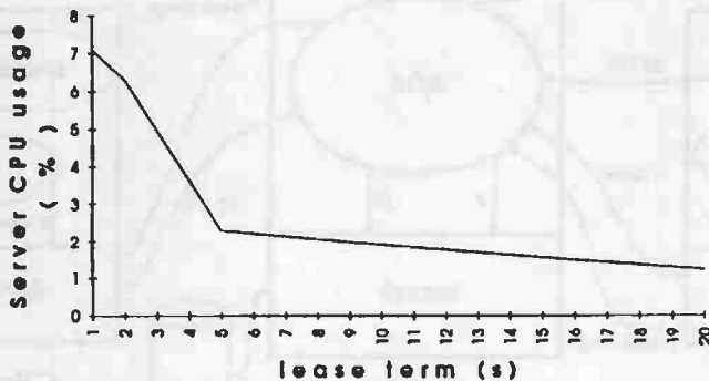
Figure 5: CPU load \times lease term
