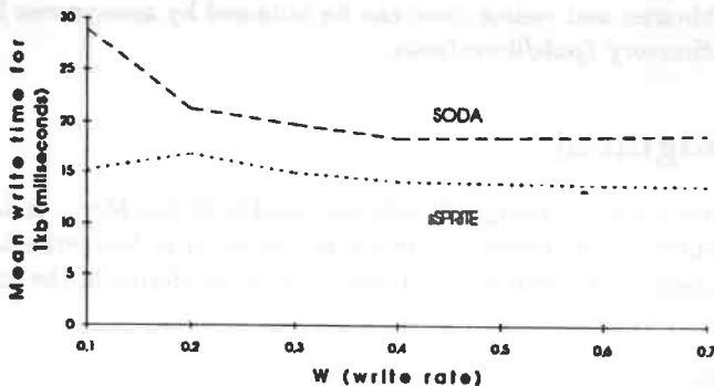
Figure 7: Elapsed time to write 1Kbyte
