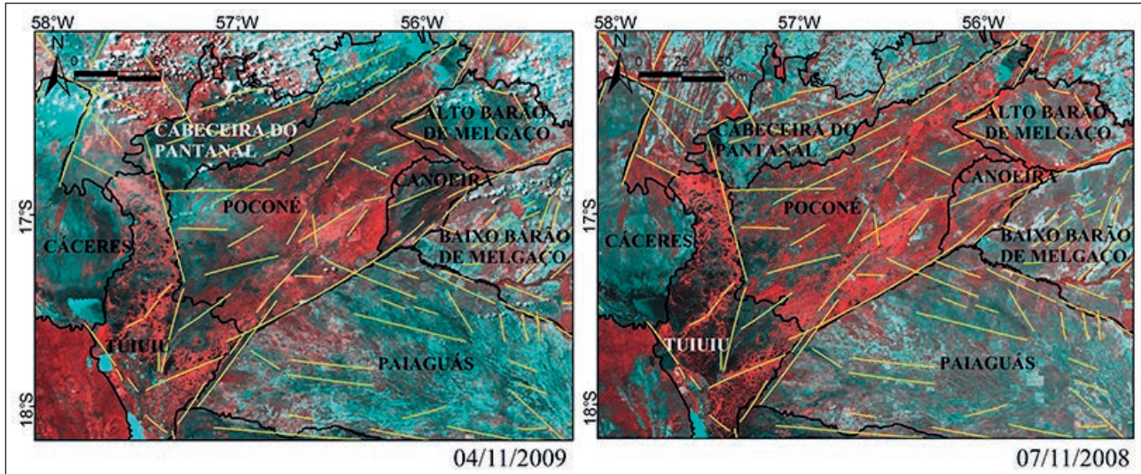
Figure 7 The Poconé Region is one of the first ones to be flooded. Observe that the flooding limits are coincident to the lineaments shown as yellow lines - MODIS images (NASA, 2008, 2009).
