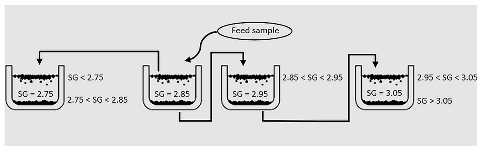
Figure 3 Procedure of the sink and float test.
