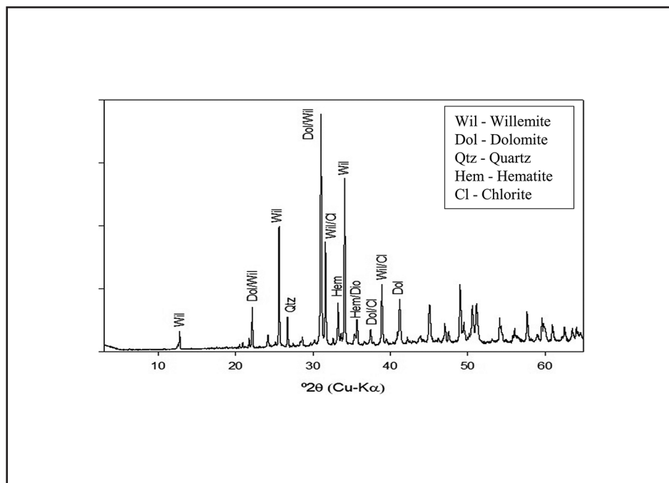
Figure 5 Diffraction pattern of the zinc ore sample.
