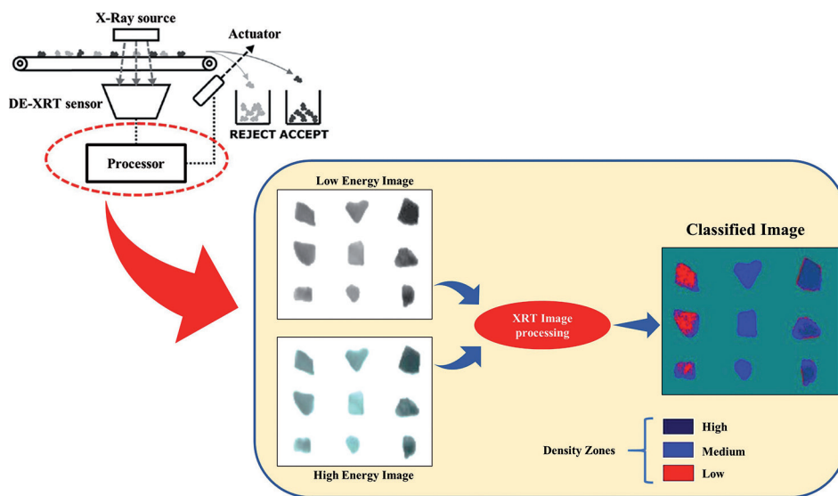
Figure 2 Image processing in the sorter. Adapted from Ketelhodt, 2012.
