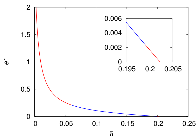
Figure 2. Fixed-point values of the density of engineers e^* as function of the decay probability \delta at the transition line \alpha = \delta/(r-1) for r = 4 and \rho = 0.005 . The fixed point is stable in the red segment of the curve and unstable in the blue segment. The inset shows that the finite-engineers fixed point becomes stable again close to the point where it vanishes ( \delta_c \approx 0.202 ), indicated by the red bullet in Figure 1.
