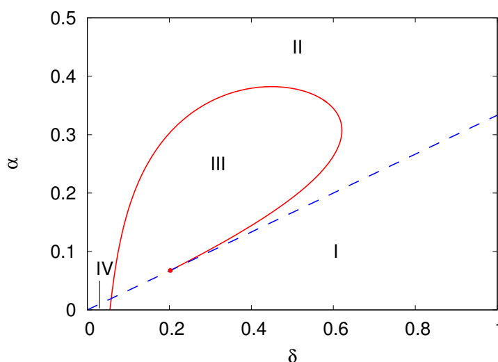
Figure 1. Regions in the space of the parameters (\delta, \alpha) where the fixed points e^* = 0 and e^* > 0 are locally stable for r = 4 and \rho = 0.005 . The zero-engineers fixed point is stable in regions I and IV, whereas the finite-engineers fixed point is stable in regions II and IV. Hence region IV, which occurs for \alpha < \delta/3 and \delta < 0.055 , is a region of bistability. The dashed blue line \alpha = \delta/3 delimits the region of stability of the zero-engineers fixed point. Region III is characterized by the oscillatory solutions. The red bullet indicates the value of \delta beyond which the transition over the dashed line is continuous.
