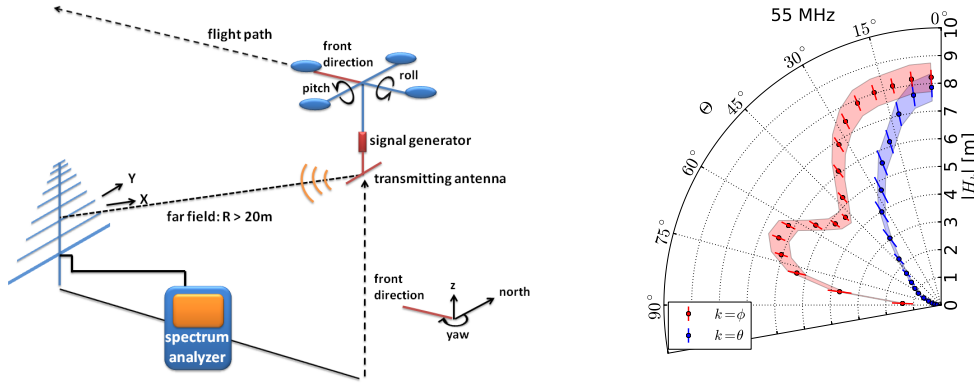
Figure 2: (left) LPDA calibration setup using an octocopter. The orientation of the octocopter is described by the yaw (twist of front measured from north in the mathematically negative direction) and the tilt by the pitch and the roll angles. [16] (right) Magnitude of horizontal and meridional LPDA VEL magnitudes (dots) and the flight-dependent uncertainties (error bars) as a function of the zenith angle in 5° bins at 55 MHz. The colored bands describe the corresponding constant systematic uncertainties. [16]
