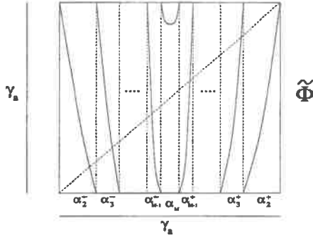
Figure 2: First return map in \gamma_a .
