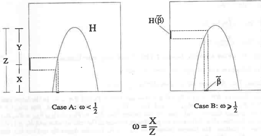
Figure 9: Two cases for the position of \tilde{\beta} .
