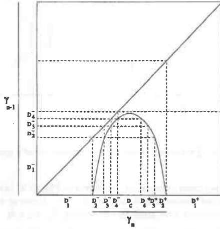
Figure 5: Fundamental domains beneath renormalization.
