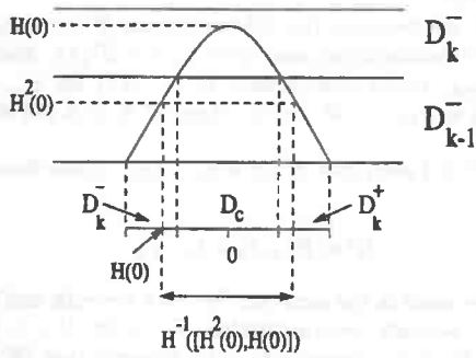
Figure 6: Detail of the critical region beneath renormalization.
