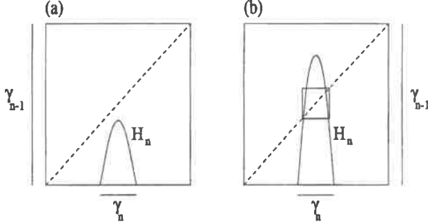
Figure 4: Two possibilities for the critical value's position.
