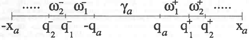
Figure 8: Partition of I_a .
