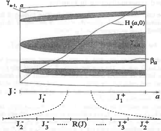
Figure 3: Parameter dependence of the critical value and the domain of \Phi_n .
