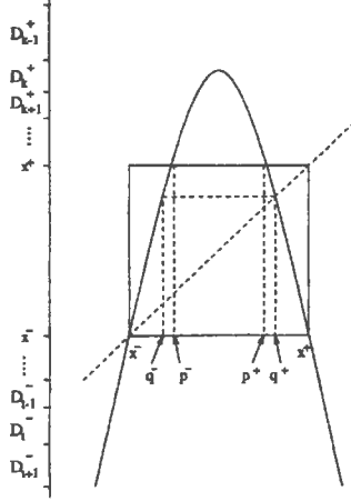
Figure 7: Fundamental domains beyond renormalization.
