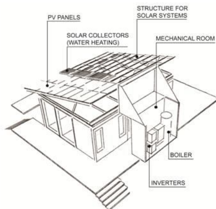
Figure 4: Solar Systems for a Solar House
