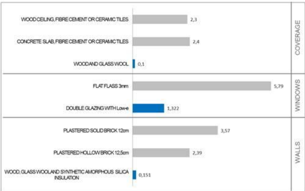
Figure 2: Materials Thermal Transmittance Values (kW/m²K)
