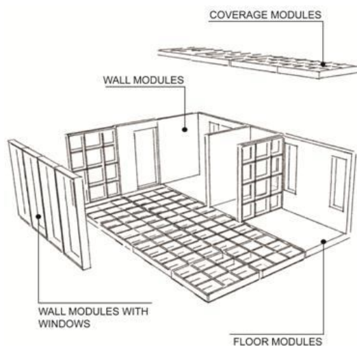
Figure 3: Modular System of Forming an Adaptive Solar House
