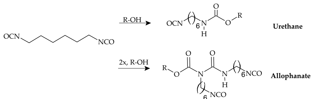
Figure 2. Main reactions of prepolymer in the curing process [30], modified by the authors.
