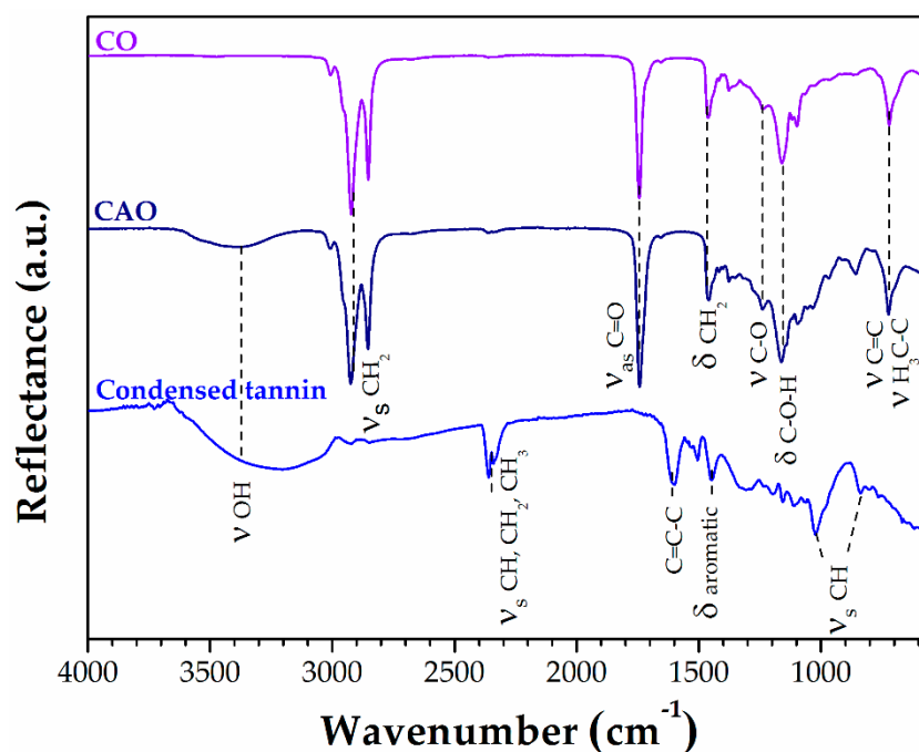
Figure 3. FTIR-ATR spectra for the crambe oil, CO (—), castor oil, CAO (—) and condensed tannin (—).
