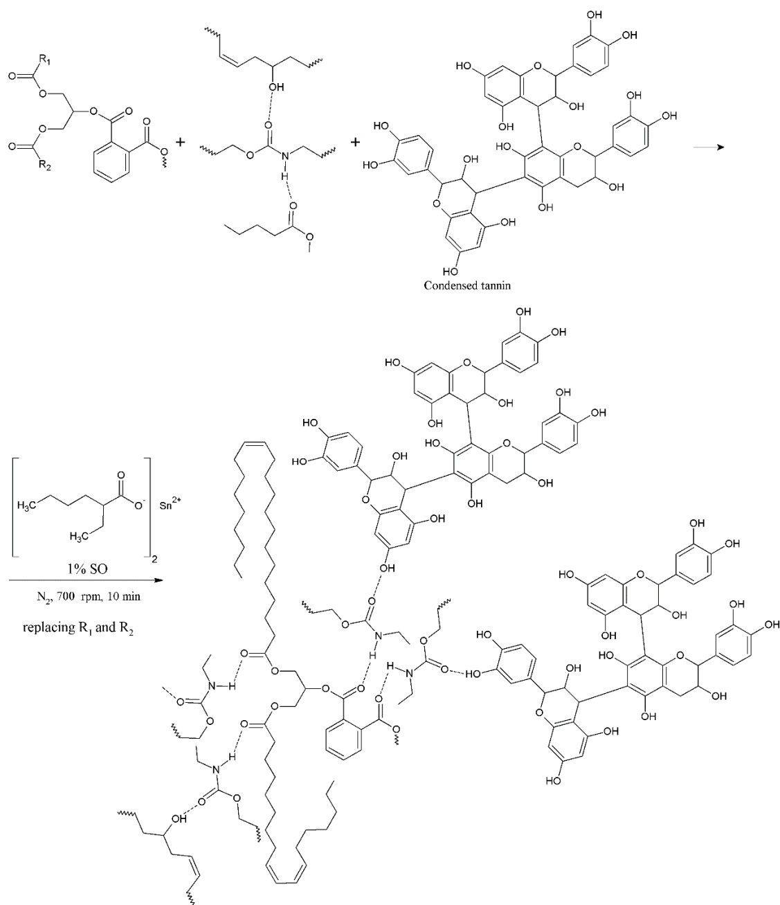
Scheme 6. Preparation of PU-modified resin.
