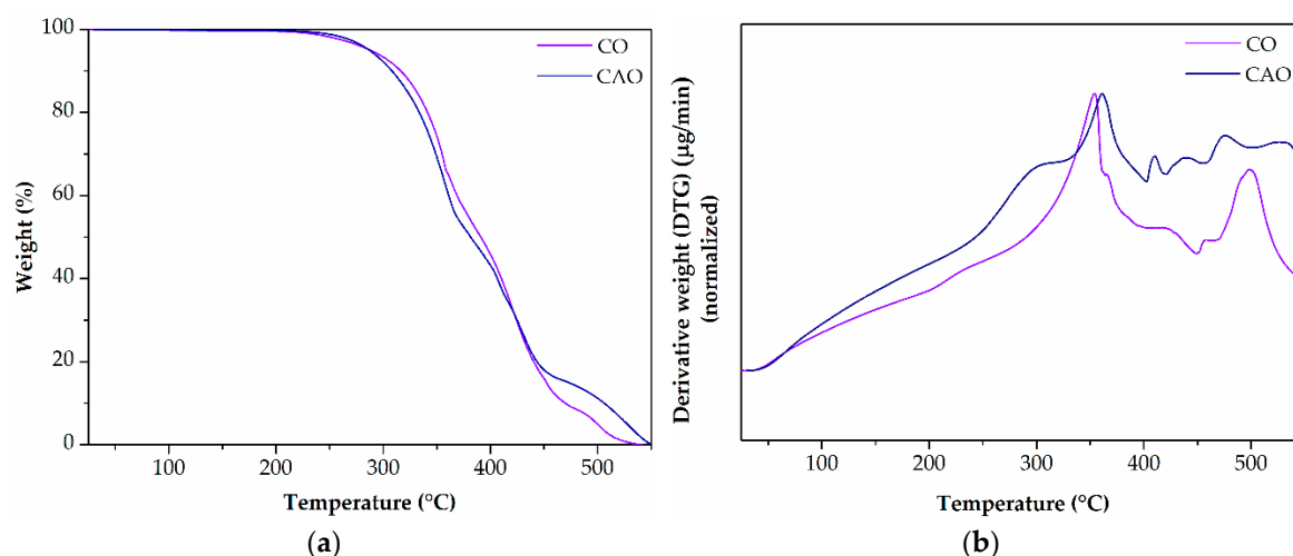
Figure 4. TGA weight loss (a) and derivatives of TGA data (b) of crambe oil, CO (—), castor oil, CAO (—).
