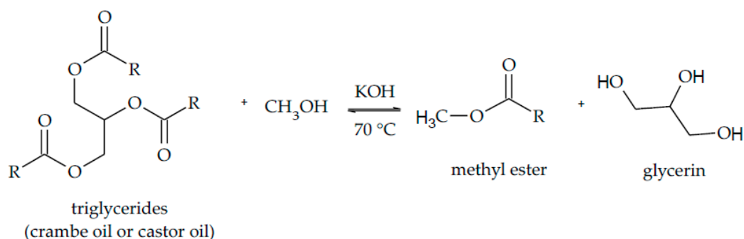
Scheme 1. Transesterification of vegetable oils to form methyl esters.
