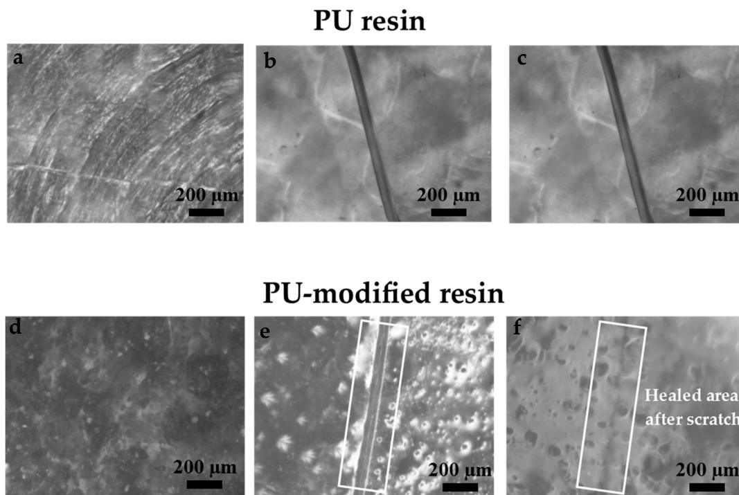
Figure 11. OM images of PU and condensed tannin-modified PU monoliths for the prepared surfaces (a,d) and after applying an artificial defect before (b,e) and after 4 h of immersion in deionized water (c,f).
