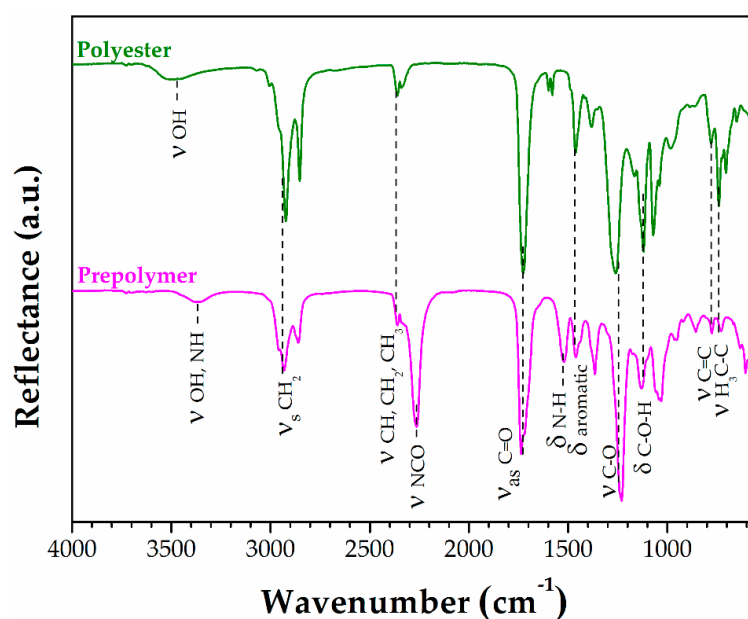
Figure 6. FTIR-ATR spectra for the polyester (—) and prepolymer (—).
