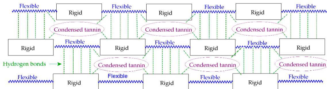
Figure 13. Scheme of hydrogen bonds between flexible and rigid segments of PU and hydrogen bonds between tanning and both segments.
