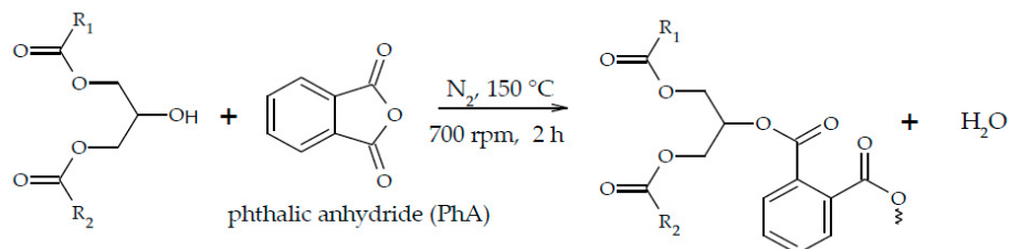
Scheme 3. Reaction that occurs with all products formed in Scheme 2, especially with the -OH for polyester formation.
