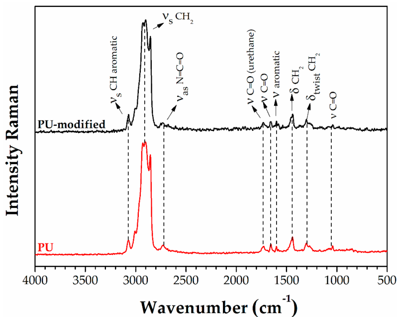
Figure 10. Raman spectra for the PU-blank and PU-modified (with intensity normalized).
