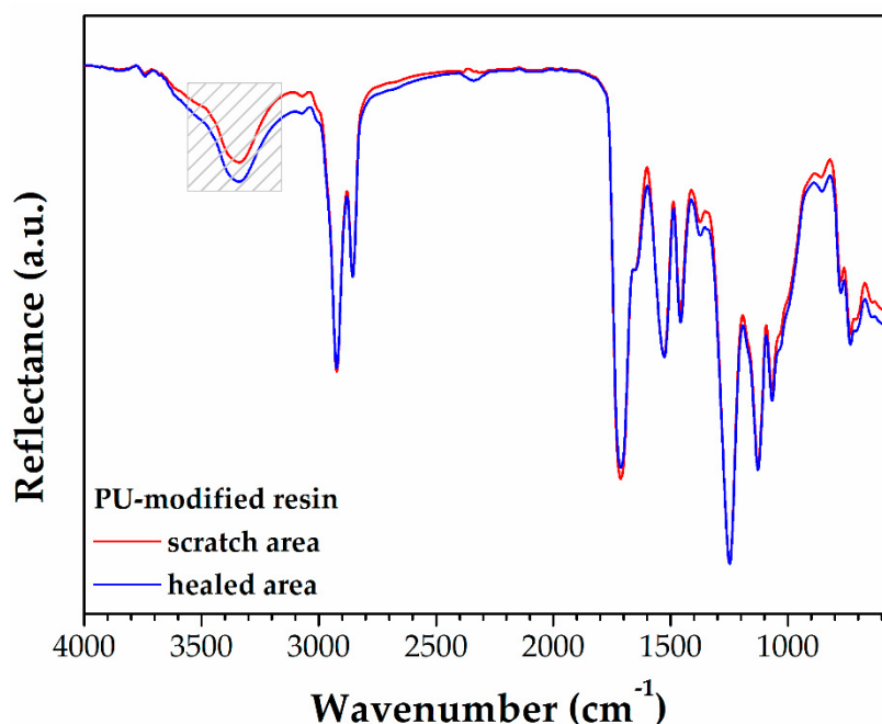
Figure 12. FTIR-ATR spectra of the modified-PU monolith with artificial defect and after having the defect repaired by immersion in water.
