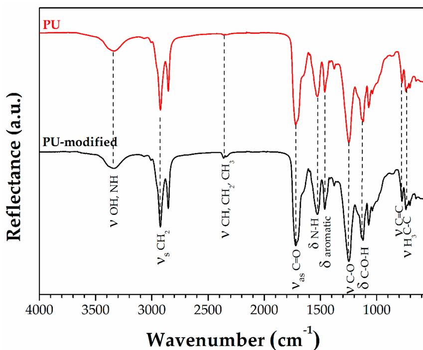
Figure 8. FTIR-ATR spectra for the PU resin (—) and PU-modified resin (—).
