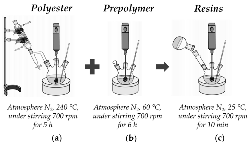
Figure 5. Reaction system for: (a) polyester, (b) prepolymer and (c) PU and PU-modified resins.
