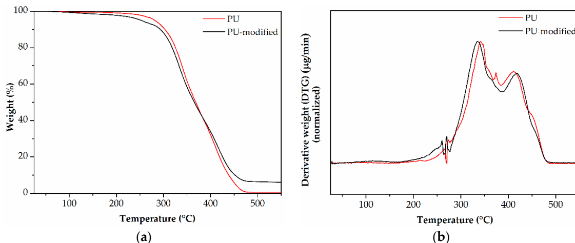
Figure 9. TGA weight loss (a) and derivatives of TGA data (b) of PU resin (—) and PU-modified resin (—).
