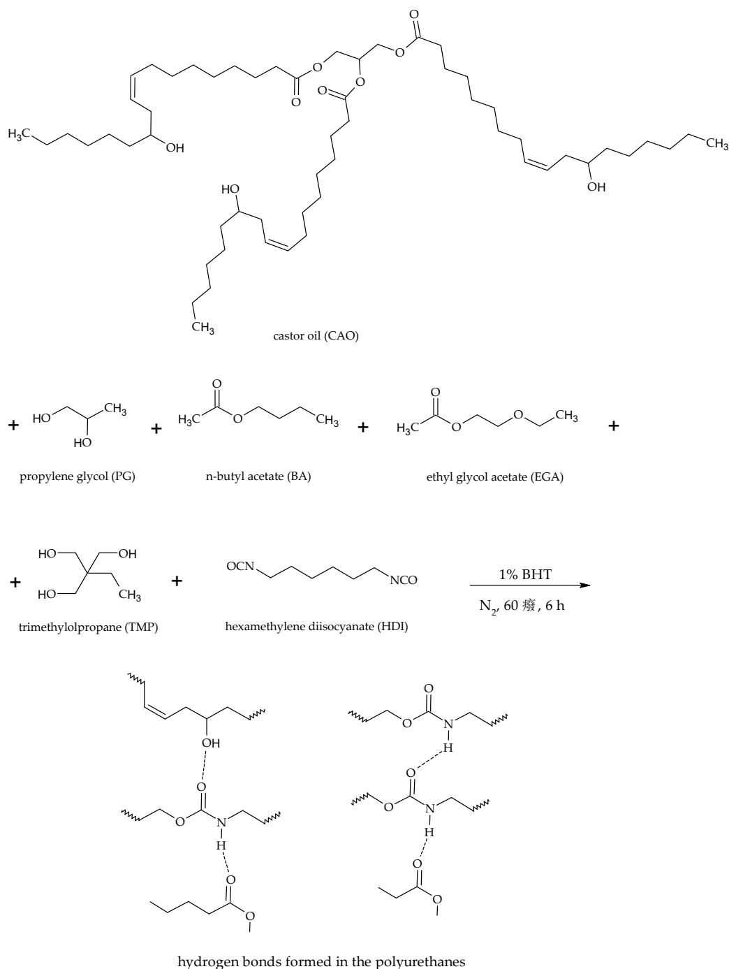
Scheme 4. Prepolymer obtaining reaction.
