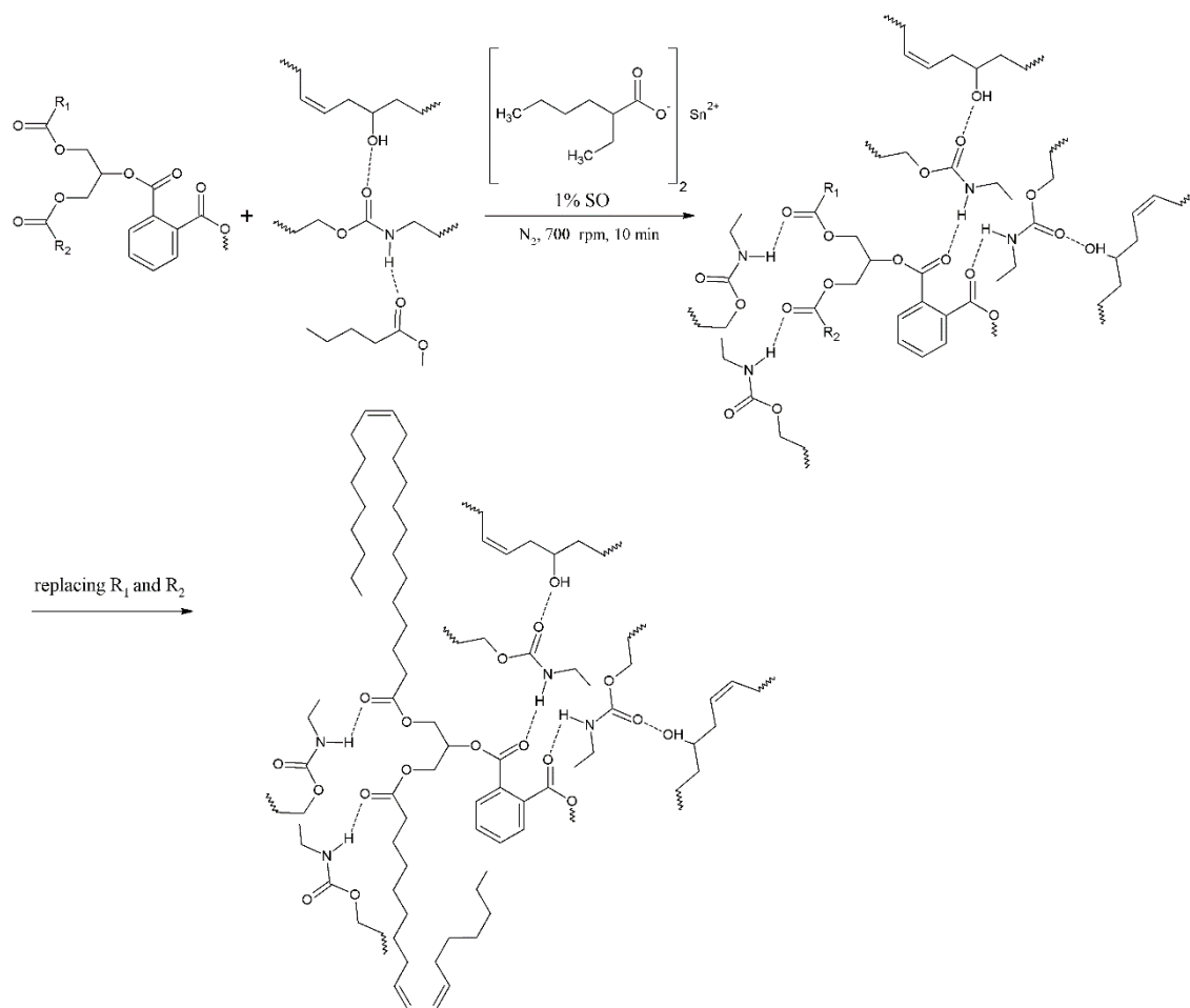
Scheme 5. Preparation of PU-resin.
