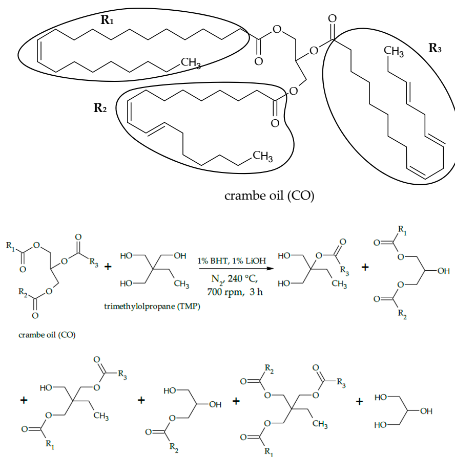
Scheme 2. First step of modification of crambe oil.
