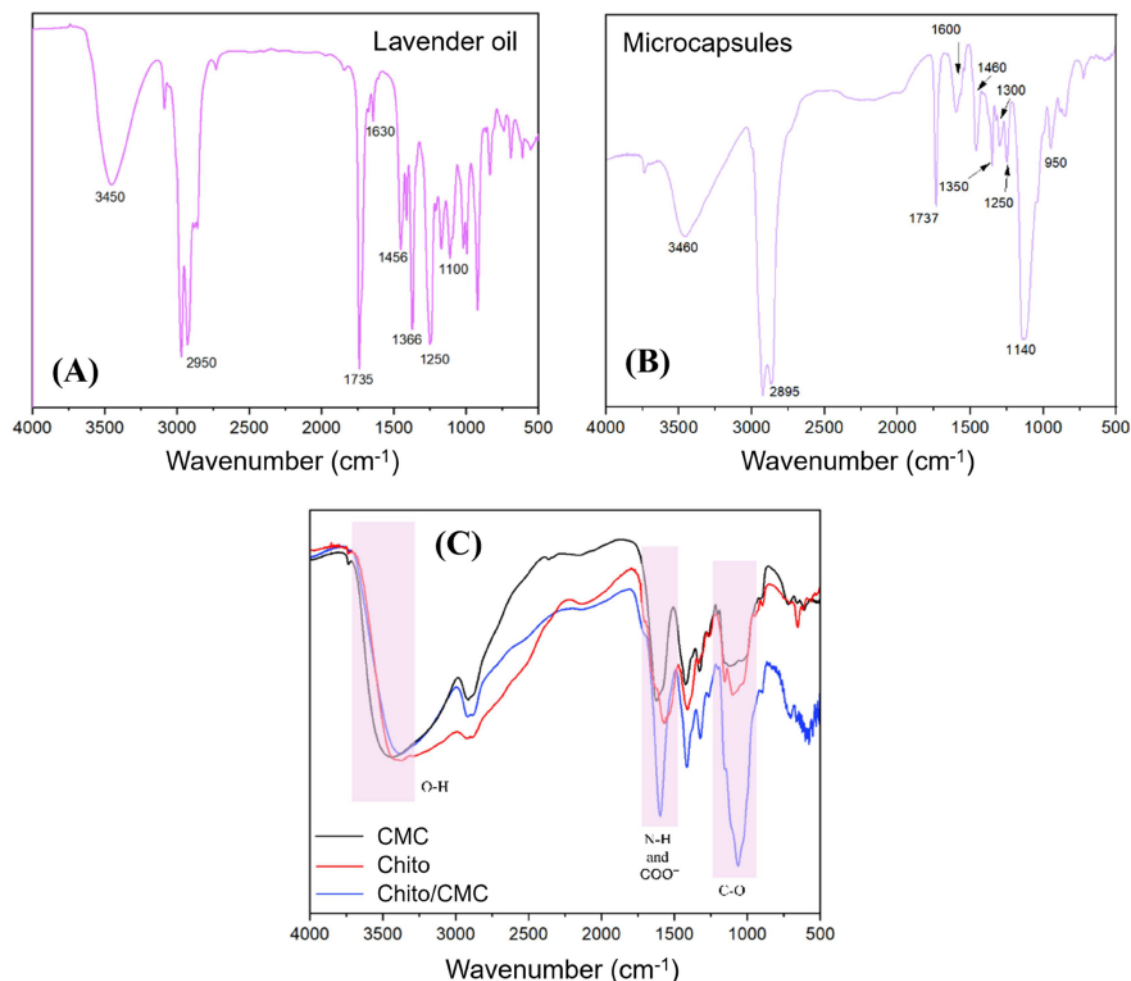
Figure 6. FTIR spectra of (A) a cast film containing lavender oil, (B) lavender microcapsules, and (C) CMC, Chito, and Chito/CMC.
