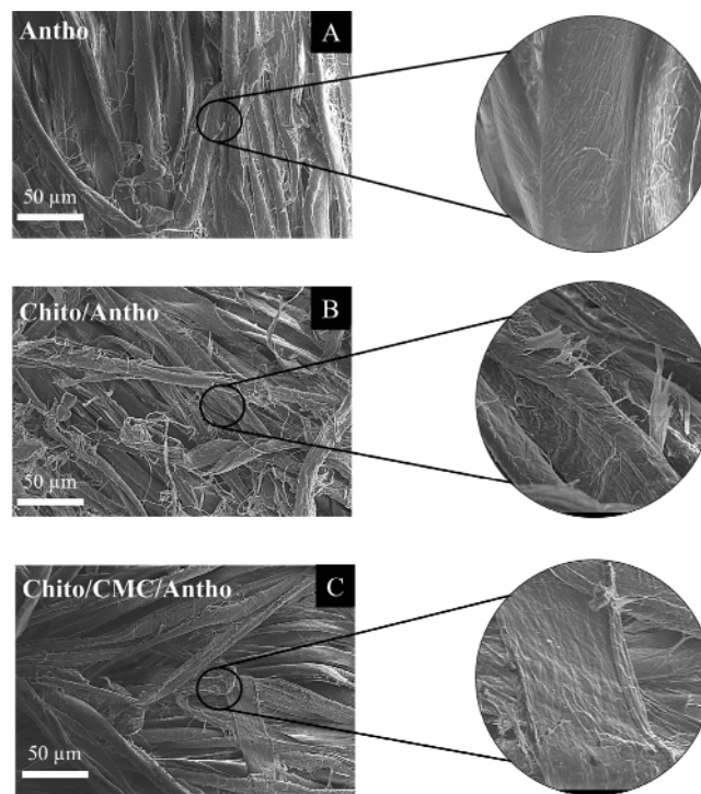
Figure 5. SEM images of cotton dyed with anthocyanin: (A) 500 \times without mordant; (B) 500 \times with chitosan as a mordant; and (C) 500 \times using chitosan/CMC as mordants.
