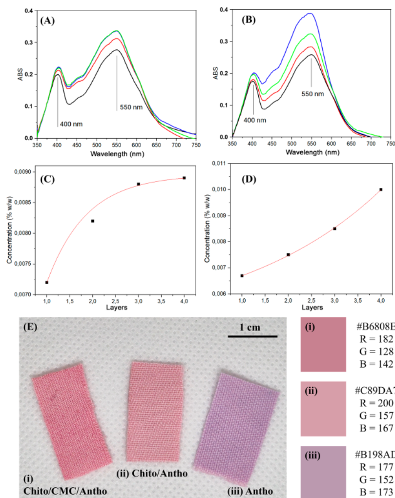
Figure 2. UV-vis spectra of fabrics dyed with anthocyanin: Using (A) chitosan and (B) chitosan/CMC as mordants with 1, 2, 3, and 4 layers. (C, D) Relationship between the anthocyanin concentration and the number of layers. (E) Digital images of fabrics with a single layer of anthocyanin using (i) Chito/CMC as a mordant, (ii) Chito as a mordant, and (iii) without a mordant. Adjacent to the image are the corresponding fabric colors with their respective RGB (red, green, and blue) color proportions.
