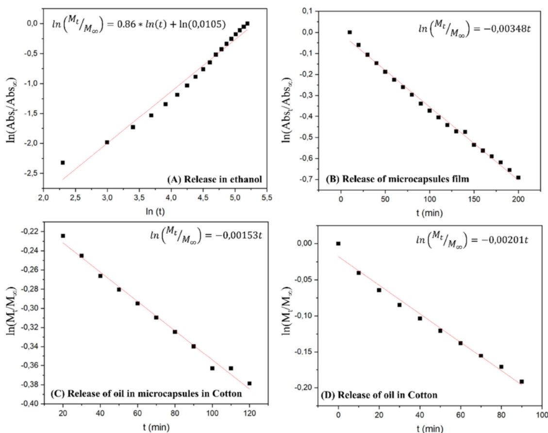
Figure 8. Analysis of lavender oil release (A) using microcapsules located in ethanol, (B) of a drop-cast film of microcapsules, (C) using microcapsules in cotton dyed, and (D) oil impregnated in dyed cotton.
