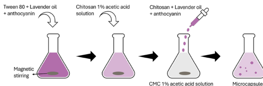
Figure 1. Illustrative scheme of the synthesis of chitosan and CMC microcapsules containing lavender oil and anthocyanin.
