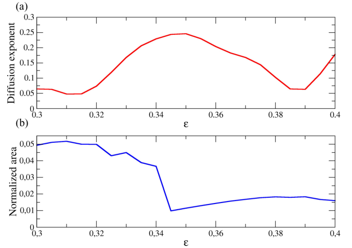
FIG. 14. In (a) and (b) we show, respectively, the plot of the diffusion exponent (red line) and normalized area of the main island (blue line) vs. parameter \varepsilon of an oval billiard.
