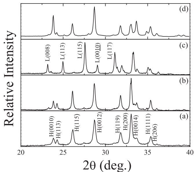
Fig. 4. X-ray diffraction patterns taken from the pre-reacted Bi-2223 powder (pristine powder) (a), and powders obtained after crushing the SPS pellets H1 (b), H2 (c), and G1 (d). The reflections belonging to the Bi-2223 (H(hkl)) and Bi-2212 (L(hkl)) phases are marked by Miller indexes in (a) and (c), respectively.
