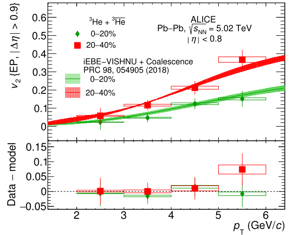
Fig. 8. Elliptic flow of (anti-) ^3\text{He} measured in the centrality classes 0–20% and 20–40% in comparison with the predictions from a coalescence model based on phase-space distributions of protons and neutrons generated from the iEBE-VISHNU hybrid model with AMPT initial conditions [13]. The model predictions are shown as lines and the bands represent their statistical uncertainties. The differences between data and model are shown in the lower panel for both centrality classes. The statistical uncertainties of the data and the model are added in quadrature. Vertical bars and boxes represent the statistical and systematic uncertainties, respectively.
