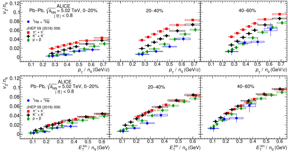
Fig. 6. Comparison between the elliptic flow of pions, kaons, protons, and (anti-) ^3\text{He} divided by the number of constituent quarks ( n_q ) as a function of p_T/n_q (upper panels) and transverse kinetic energy per constituent quark E_T^{\text{kin}}/n_q (lower panels) for the centrality classes 0–20% (left), 20–40% (middle) and 40–60% (right). See text for details. Vertical bars and boxes represent the statistical and systematic uncertainties, respectively.
