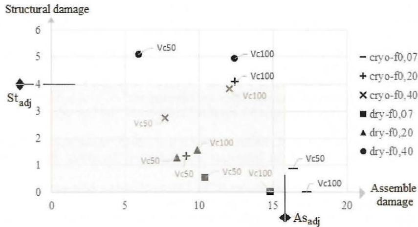
Figure 6. The results of damages and thresholds for Structural (St adj ) and Assemble damages (As adj ).
