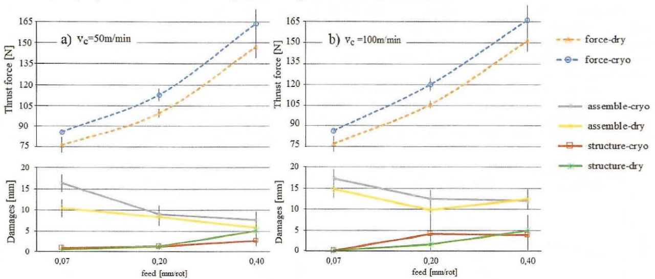
Figure 4. Damages Vs Thrust force a) at v_c=50 m/min and b) at v_c=100 m/min
