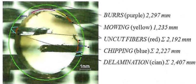
Figure 2. An example of Global Damage measurement.
