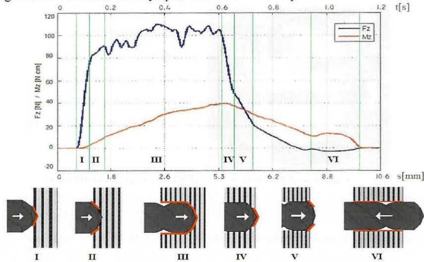
Figure 3. Thrust force and torque at each step (I to VI) of drilling
