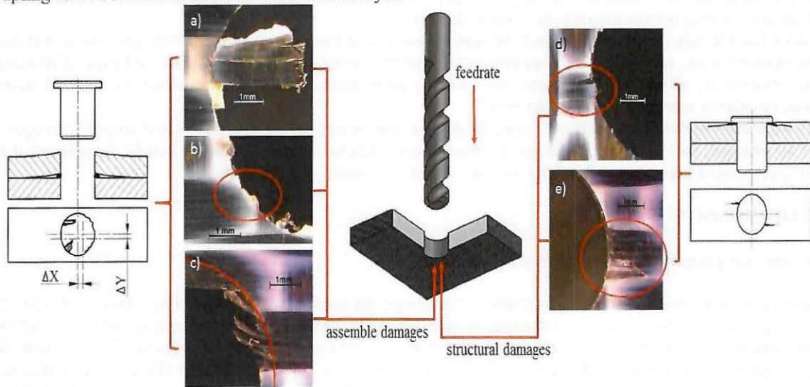
Figure 1. Types of damage at hole exit a) uncut fibers, b) burr, c) mow, d) chipping and e) spalling
