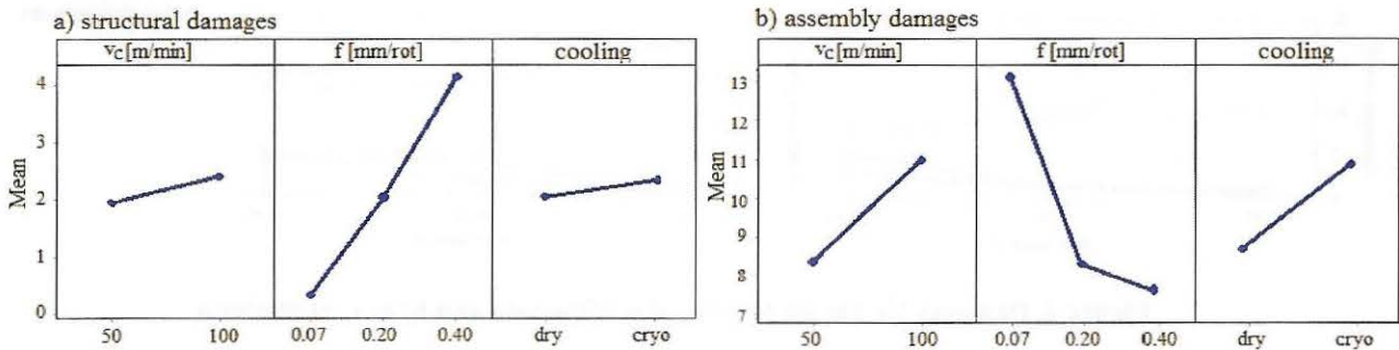
Figure 5. (a) Structural damages and (b) assembly damages a function of rotation, feedrate and cooling type.
