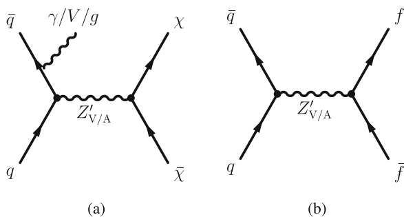
Fig. 2 Representative Feynman diagrams of the dominant production and decay modes for the V/AV model
