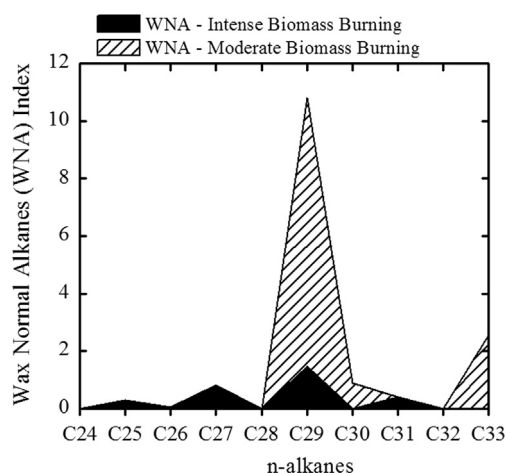
Fig. 4. Results of source distribution of WNA index during intense and moderate biomass burning periods.
