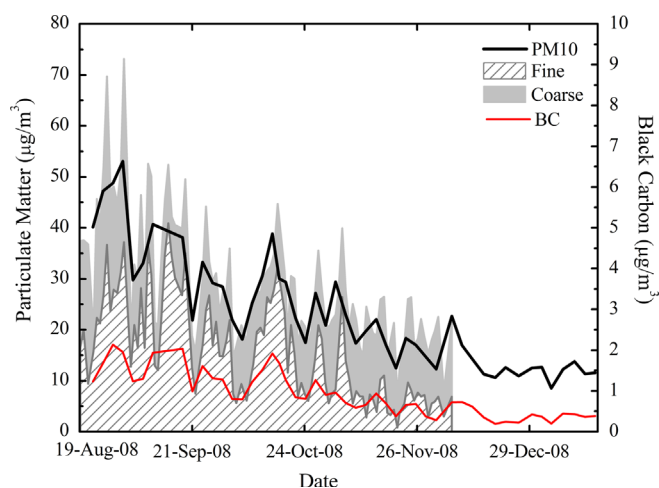
Fig. 3. Results of the mass concentration of coarse and fine fractions, PM 10 and BC emissions from biomass burning in Alta Floresta.
