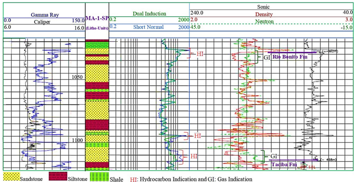
Fig. 4. Hydrocarbon indication below 1029 m
