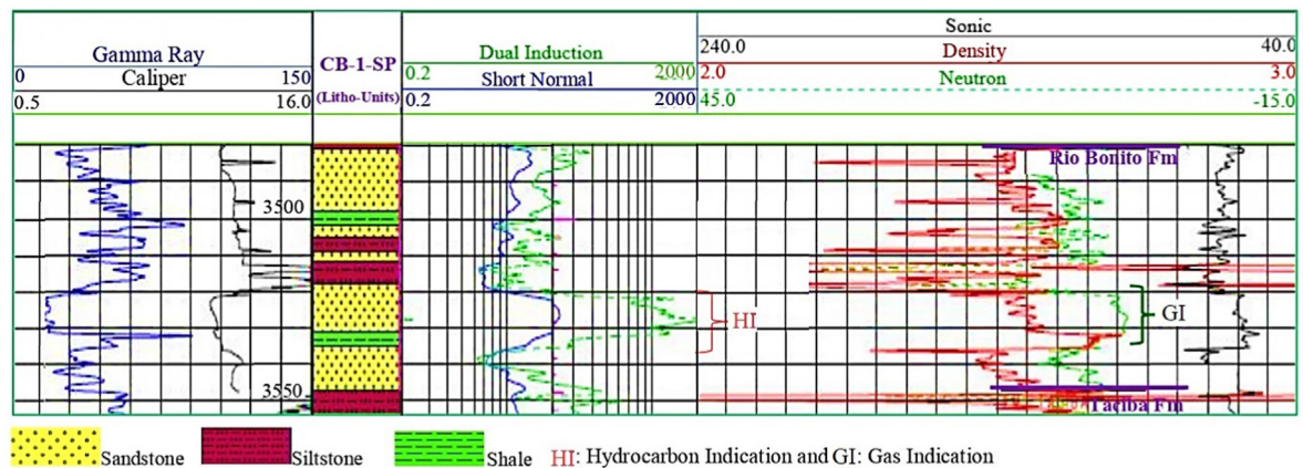
Fig. 5. Gas indication below 3520 m
