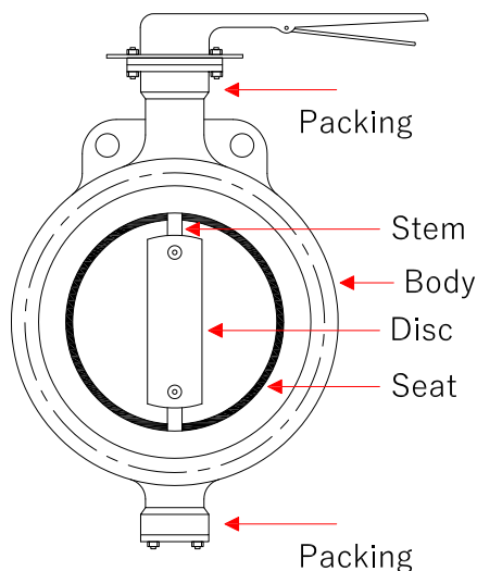
FIGURE 3. Schematic diagram of a butterfly valve.
