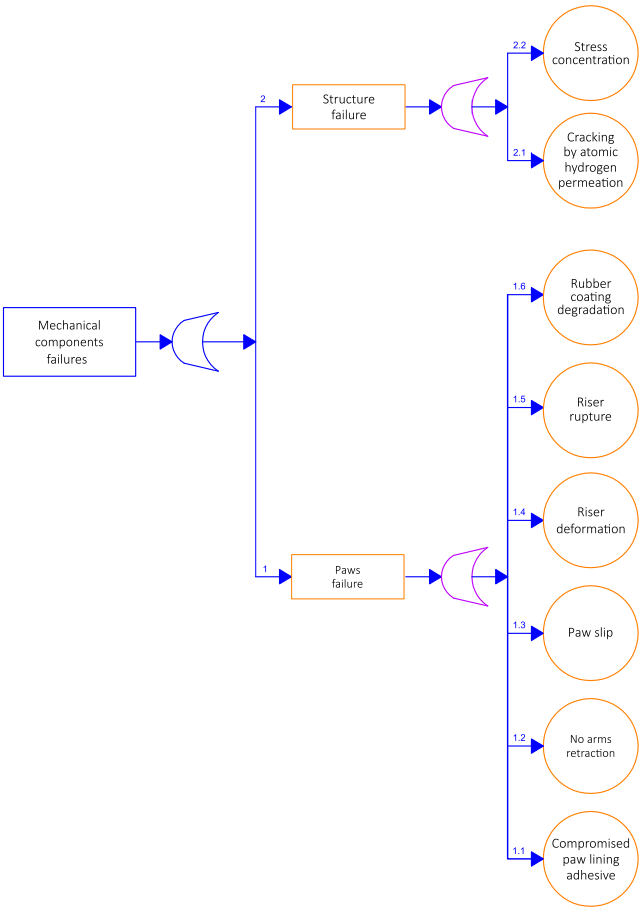
FIGURE 9. FTA of in-pipe robot traction system failure.
