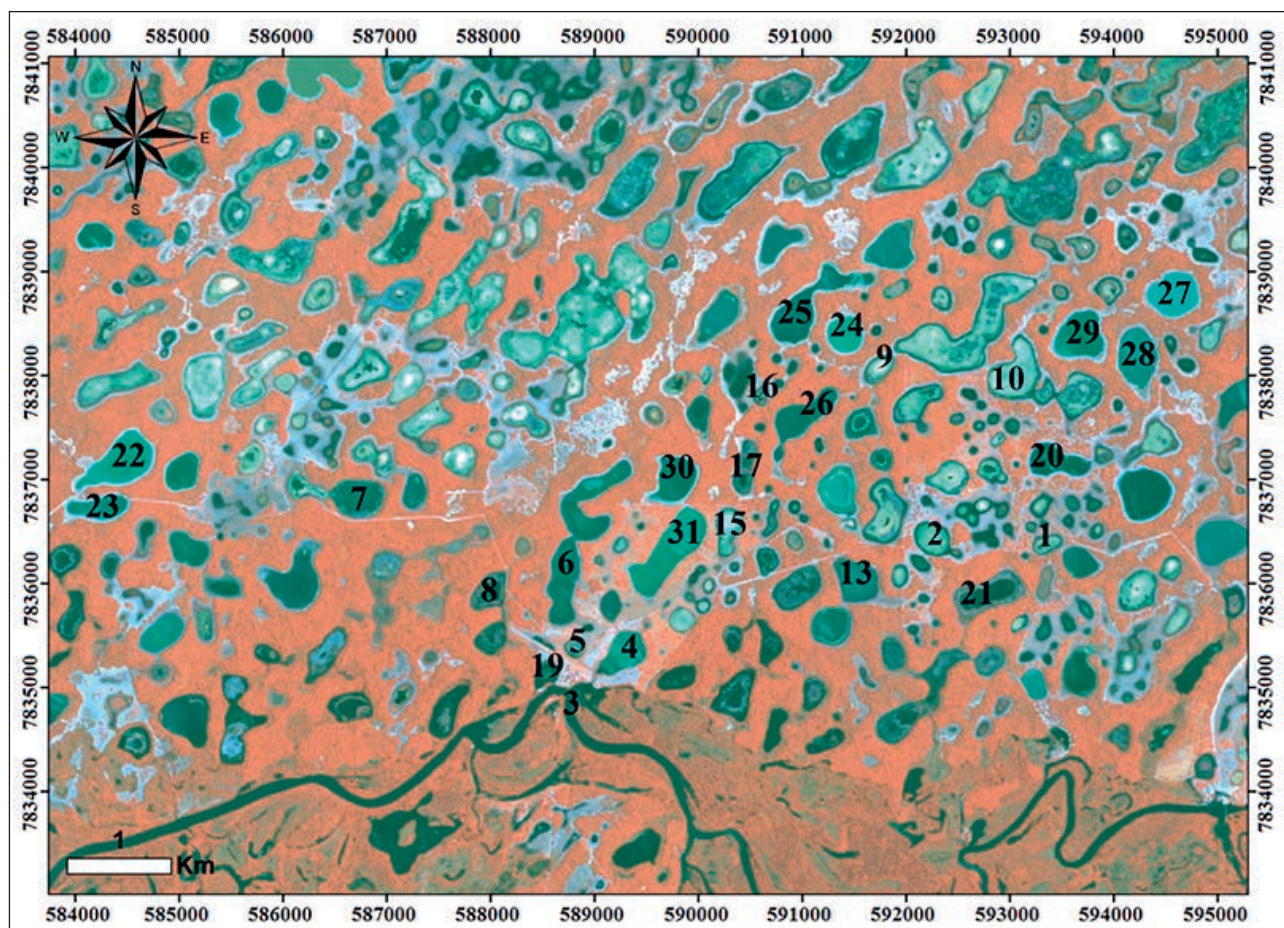
Figure 2 Location and id number of the sampled lakes in the field during 2012 and 2013. In an ALOS satellite image, AVNIR-2 sensor, the water has a blue-green color and the vegetation appears in red. In the white color are the outcrops of the sandy substrate.
