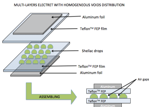
Fig. 1. Assembling process of multi-layer electrets with homogeneous air gaps. Shellac drops are employed as spacers between two Teflon™-FEP films thus forming regular cavities, as indicated in the cross-section representation.
