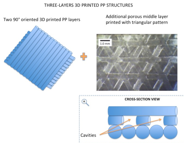
Fig. 10. 3D-printed model for a three-layer design, with a magnified view from the triangular pattern formed by increasing the layer porosity. And a cross-sectional representation of the cavities. 18
