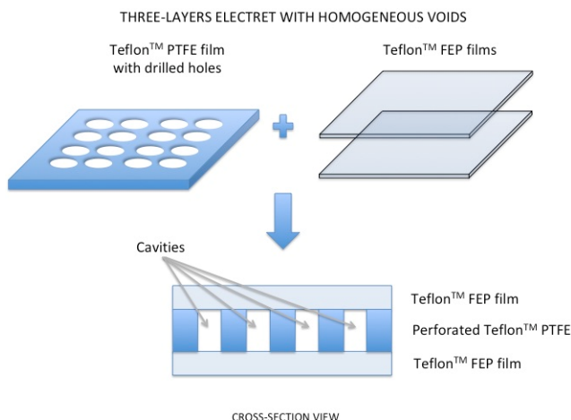
Fig. 3. Schematic representation of the assembling process for producing three-layer electrets with a perforated middle. 10
