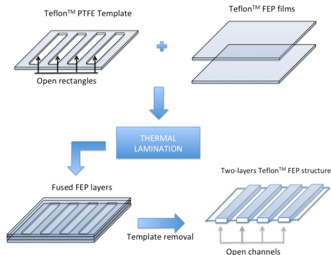
Fig. 4. Schematic representation of the method for producing open-tubular channels FEP structures using thermal lamination and a PTFE template. 11
