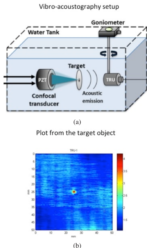
Fig. 12. (a) Vibro-acoustography setup assembled with a hydrophone built with a ferroelectret transducer (TRU) for capturing the target vibrations. (b) Resulting image of a small spherical object produced from the scanning with the TRU. 28
