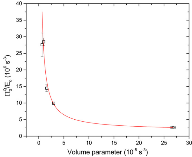
Figure 3. \Pi versus the \mathcal{V} diagram of a trapped Bose–Einstein condensate in the limit for T = 0 . The pressure parameter for T = 0 and N = 0 , \Pi_0(N = 0) , divided by E_0 , as a function of the volume parameter. The fitting was done with a curve proportional to \mathcal{V}^{-1} .
