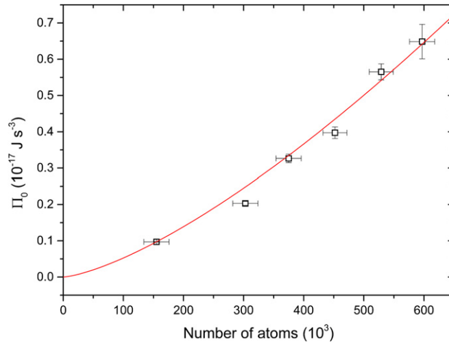
Figure 2. The pressure parameter for T = 0 ( \Pi_0 ) as a function of the total number of atoms ( N ). In the case of this figure, the volume parameter was kept equal to \mathcal{V}_4 = 3 \times 10^8 \text{ s}^3 . The solid red curve is the obtained \Pi_0(N) built from the \Pi_0^{\text{TF}}(N) fit.
