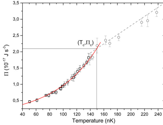
Figure 1. \Pi versus T phase diagram of a trapped bosonic cloud. Pressure parameter ( \Pi ) as a function of temperature ( T ) for N = 3 \times 10^5 and \mathcal{V}_4 = 3 \times 10^8 \text{ s}^3 . The change in the behavior of \Pi is due to the appearance of a BEC fraction that allows us to determine the critical point ( T_c, \Pi_c ). An exponential extrapolation below T_c gives the value of the pressure parameter at the limit of T \rightarrow 0, \Pi_0 . The error bars represent the statistical error on average.
