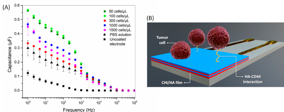
Figure 4. (A) Capacitance spectra for CHI/HA functionalized electrodes after exposure to different concentrations of tumor cells (50–1500 cells/ \mu\text{L} ). The spectrum of an uncoated electrode is also shown. (B) Schematic representation of tumor cell adhesion mediated by CD44-HA interaction in CHI/HA functionalized electrodes.
