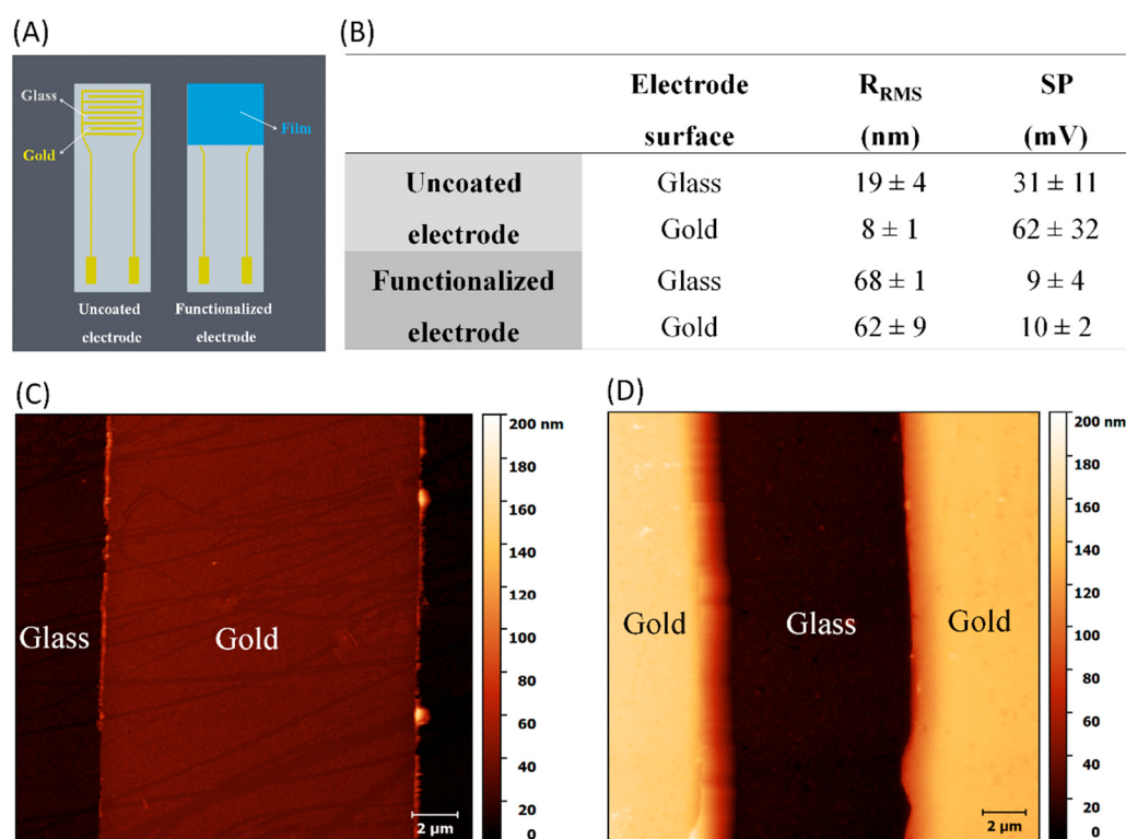
Figure 2. (A) Schematic representation of the electrode functionalization. (B) Average measurements of root mean square roughness ( R_{RMS} ) and surface potential (SP) for electrodes before and after layer-by-layer (LbL) functionalization. Atomic force microscopy (AFM) images for interdigitated electrodes (C) before and (D) after chitosan (CHI)/hyaluronan (HA) film deposition.
