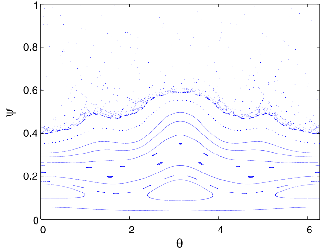
Fig. 2. (Color online.) Poincaré section of the Revtokamak with \varepsilon = 6/2\pi .
