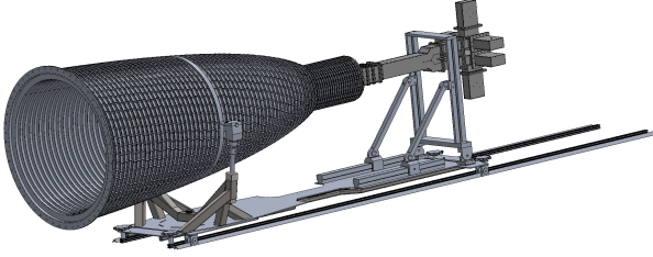
Fig. 7. Horn support system, designed to move the horn up and down according to the calculated positioning values. In the case of the double-rectangular and triple-rectangular the maximum value is \pm 30 cm from a central reference position. In the case of the rectangular arrangement, the value is \pm 42 cm. This cell support allows for the positioning of all horns in their optimal location as described in this paper. This is further discussed in the companion study in Paper (II) (Wuenschel et al. 2022).
