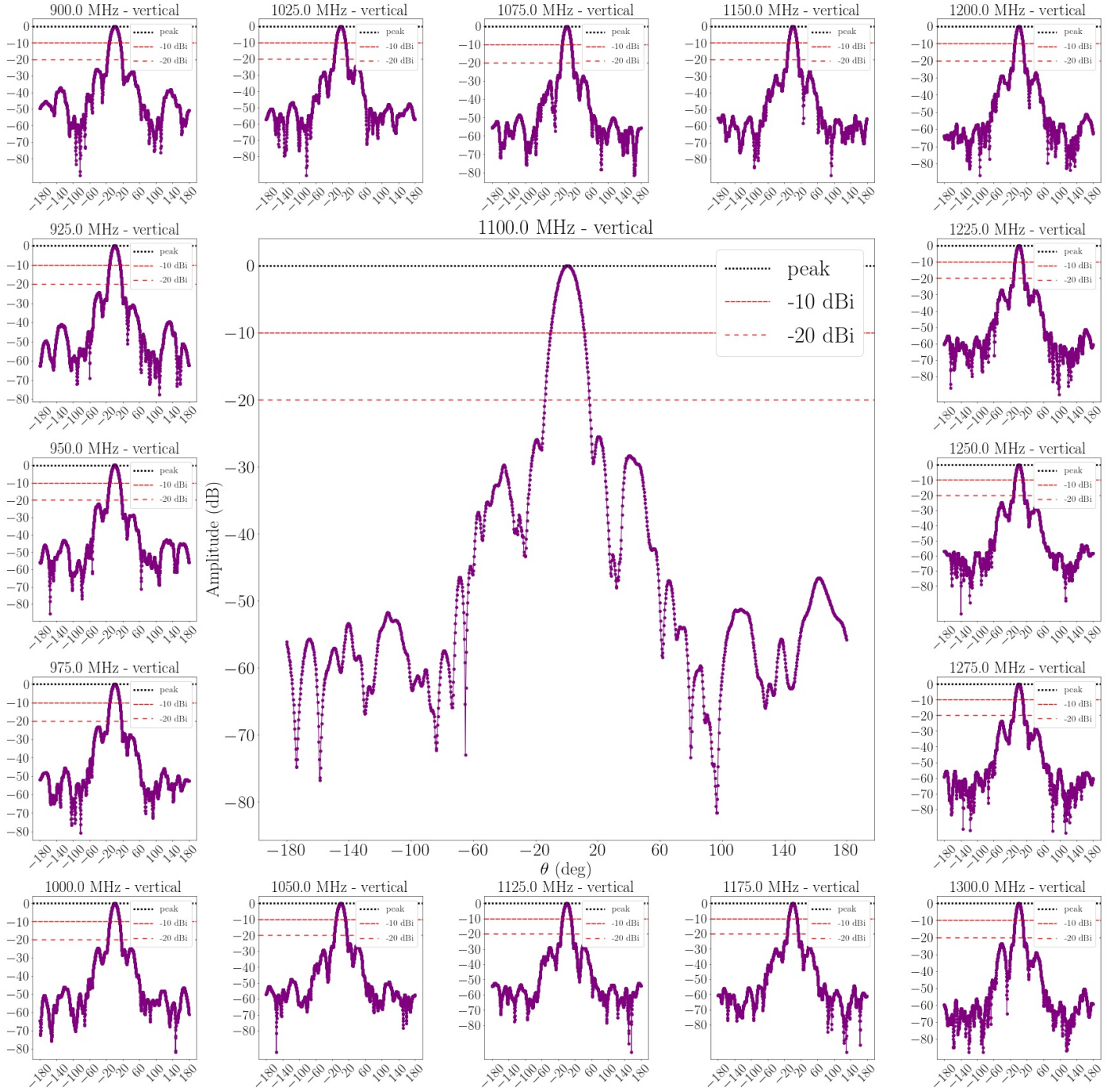
Fig. C.2: Plots from the horn beam measurements from Wuenschel et al. (2020) used to obtain the 10-20 dB attenuation angles as a function of frequency for a vertically polarized input signal. For each plot the intensity is attenuated by 10 dB (red dashed line) and 20 dB (sparse red dashed line) in relation to the peak intensity (black dashed line).
