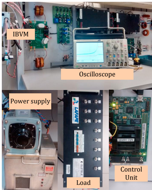
Fig. 4. The experimental test bench with a IBVM converter
