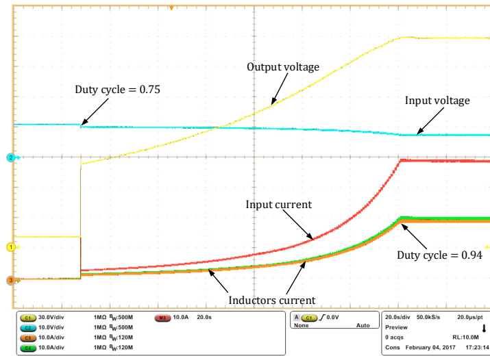
Fig. 6. IBVM converter waveforms during the duty cycle sweep between 0.75 and 0.94. The blue line is the input voltage with 10V/div, the yellow line is the output voltage with 30V/div, the orange line is the current in an inductor with 10A/div, the green line is the current in the another inductor with 10A/div and the red line is the input current with 10A/div. The time scale was 20s/div.
