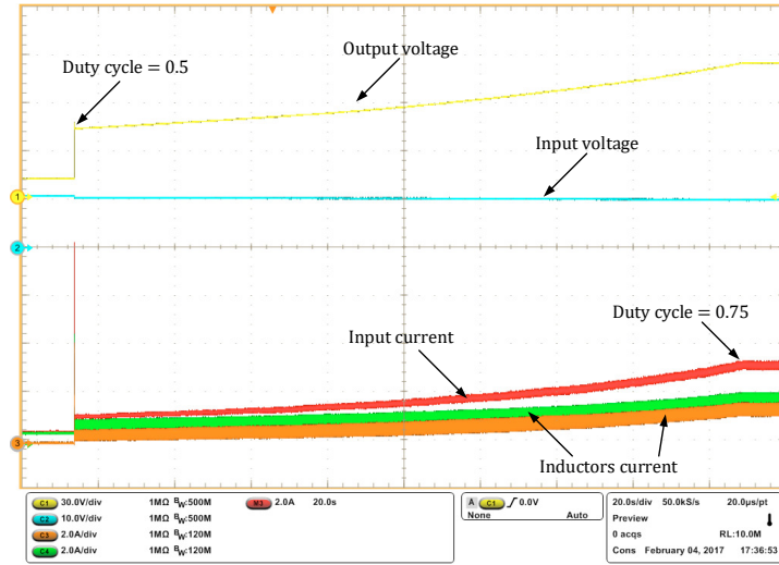
Fig. 5. IBVM converter waveforms during the duty cycle sweep between 0.5 and 0.75. The blue line is the input voltage with 10V/div, the yellow line is the output voltage with 30V/div, the orange line is the current in an inductor with 2A/div, the green line is the current in the another inductor with 2A/div and the red line is the input current with 2A/div. The time scale was 20s/div
