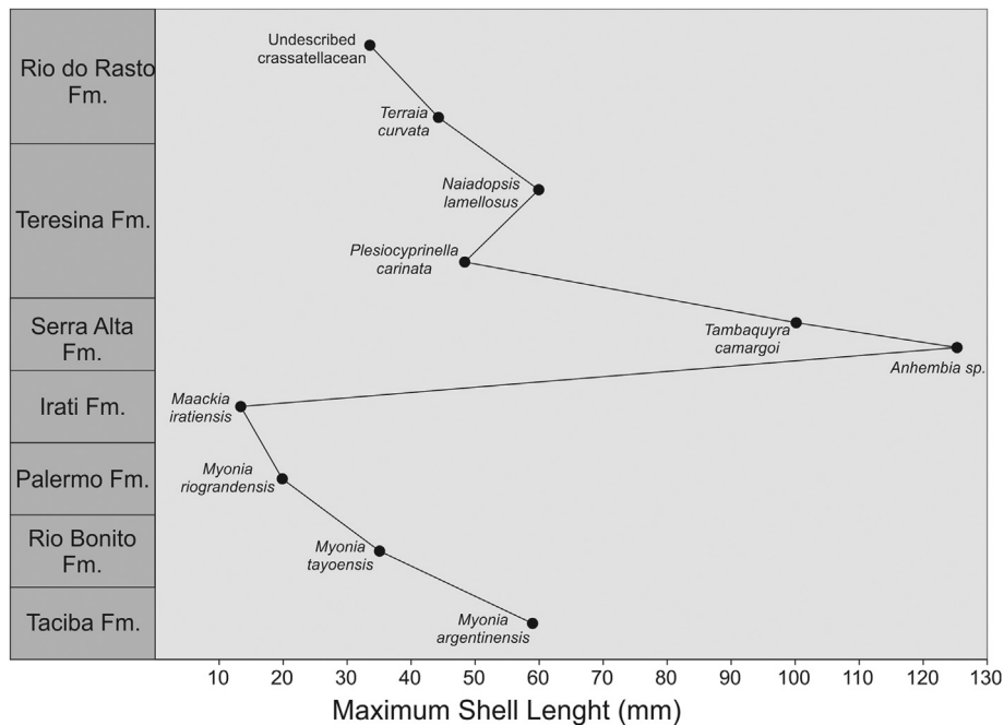
Fig. 14. Maximum length of the largest individuals recorded in assemblages of the Permian Passa Dois Group. Undescribed crassatellacean (35 mm), Terraia curvata (42.4 mm), Naiadopsis lamellosus (59.9 mm), Plesiocyprinella carinata (48.4 mm), Tambaquyra camargoi (104.5 mm), Anhembia sp. (125 mm), Maackia iratiensis (13.5 mm), Myonia riograndensis (20 mm), Myonia tayoensis (35 mm), and Myonia argentinensis (59 mm). Source of data: 2434 specimens from the scientific collection of the Department of Zoology, Institute of Biosciences, UNESP, Botucatu campus (DZP-code) and literature data in Beurlen (1957), Rocha-Campos (1970), Simões (1992), Neves et al. (2014), Simões et al. (2015). Modified from Ghilardi (1999).
