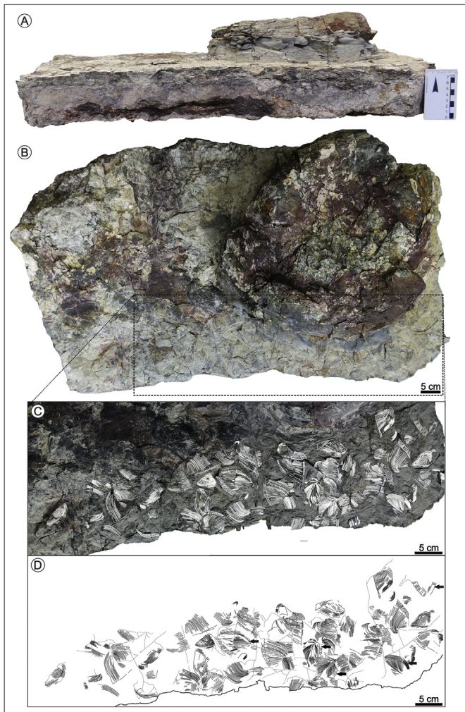
Fig. 8. General taphonomic, paleontological, and sedimentological features of the disrupted, “brecciated” carbonate bed. A– Cross-section of an 86-cm-long slab showing a well preserved low relief mound at right. B– Plan-view of the same slab. C– Mono-specific assemblage of T. camargoi at the base of the mound. D– Drawings of the shells in C.
