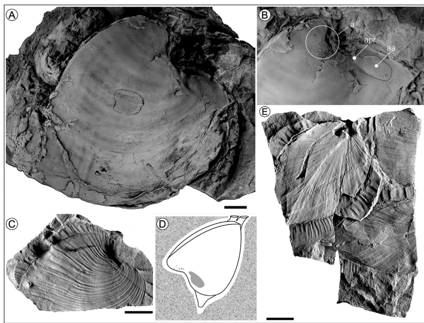
Fig. 12. Tambaquyra camargoi . A- Lateral view, internal mold, right valve of a large specimen (DZP-2250). B- Detail of specimen in A, note the large, elongated and deeply impressed anterior adductor muscle scar, as well as other muscle scars. C- Composite mold, right valve, showing the ornamentation. D- Inferred mode of life of T. camargoi . E- In situ preserved closed valves of T. camargoi at the base of a mound. a-accessory muscle scar; apr-anterior pedal retractor muscle scar, and aa-anterior adductor muscle scar. Scale bar: 1 cm.
