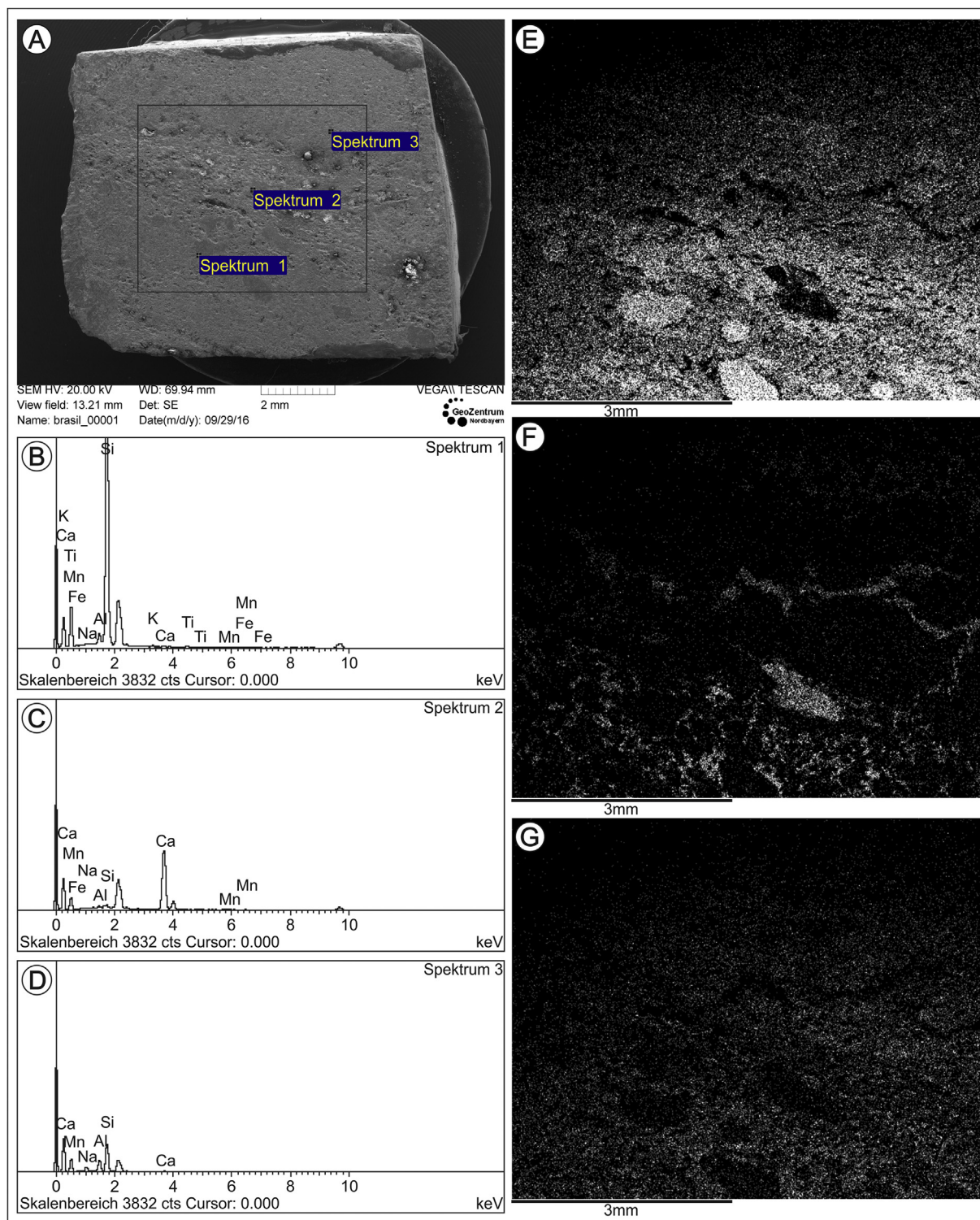
Fig. 11. SEM-EDS analysis of the lower unit of the “brecciate” carbonate. A- SEM image with positions of the three spectral analyses. B- EDS spectrum 1. C- EDS spectrum 2. D- EDS spectrum 3. E-G- Mapping results: E, Silica; F, Calcium; G, Alumina.
