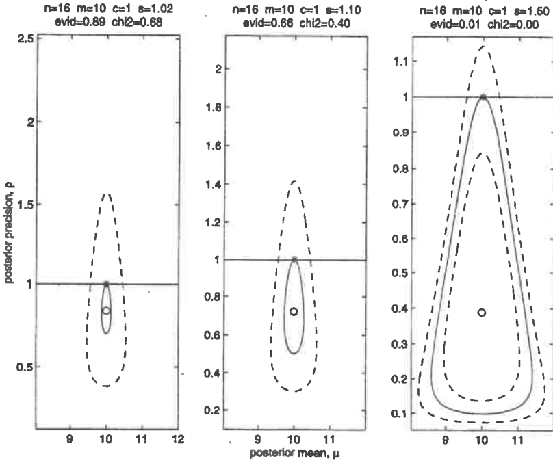
Figure 1: Tangent and other Highest Probability Density Sets
