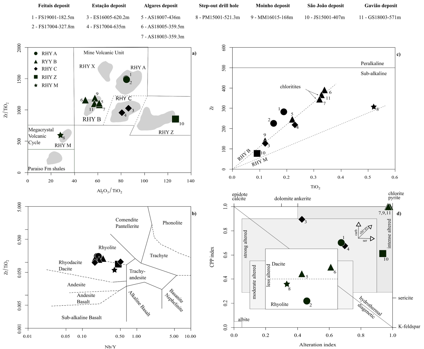
Fig. 3. Immobile element and alteration plots of the 11 geochronological samples selected in this study a) \text{Al}_2\text{O}_3/\text{TiO}_2 vs. \text{Zr}/\text{TiO}_2 , chemostratigraphic type fields (grey areas) after Barrett et al. (2008) and Barrett (2008), main volcanic units and sediments of the Paraiso Fm are schematic and highlighted by straight closed fields; b) \text{Nb}/\text{Y} vs. \text{Zr}/\text{Ti} , rock classification diagram (Winchester and Floyd, 1977) c) \text{TiO}_2 vs. \text{Zr} dashed lines, after Barrett et al. (2008), represent alteration trends resulting from gain or loss in Zr and Ti of the near-constant proportion ( \text{Zr}/\text{TiO}_2 ) chemostratigraphic types RHY B and RHY M. Peralkaline and sub-alkaline felsic fields after Leat et al. (1986); d) Alteration index vs. CPP index, alteration diagram (Large et al., 2001). Alteration boxes adapted from Giffkins et al. (2005) and Large et al. (2001). Arrows represent the apparent main alteration trends of the studied rocks.
