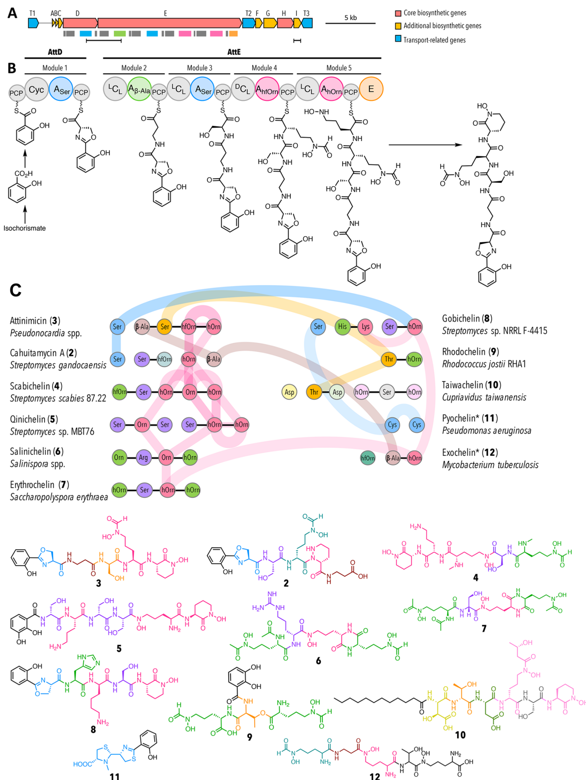
Figure 4. Bioinformatic analysis of the putative attnimicin biosynthetic gene cluster. (A) Attinimicin biosynthetic gene cluster. Colored rectangles indicate the domains shown in B. Horizontal black bars represent regions amplified for PCR-based detection of the att BGC (left) and att -like BGC (right); (B) proposed model for attinimicin biosynthesis. A, adenylation domain—amino acids in subscript indicate the monomers incorporated into the nascent peptide; PCP, peptidyl carrier protein; Cyc, cyclization domain; D CL, condensation domain that catalyzes the peptide bond between the terminal D-amino acid of the growing peptide chain and an L-amino acid to be incorporated; L CL, condensation domains condense two L-amino acids; E, epimerization domain; (C) Proposed evolutionary relatedness between the attinimicin and other siderophore NRPSs based on phylogenetic analysis of adenylation domains (for a detailed representation see Supporting Information, Figure 14). Only relationships between attinimicin and other clusters are shown. Horizontal black lines represent domains encoded on the same gene; colored vertical lines and colored horizontal connections represent domains that are evolutionarily related and/or duplicated.
