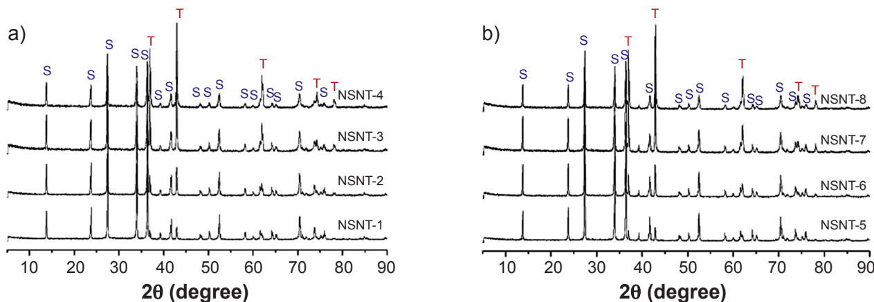
Figure 1: XRPD patterns of sintered samples at: a) 1750 °C/1 h; and b) 1815 °C/1 h. S is \beta\text{-Si}_3\text{N}_4 (PDF 33-1160) and T is TiN (PDF 87-0628).
