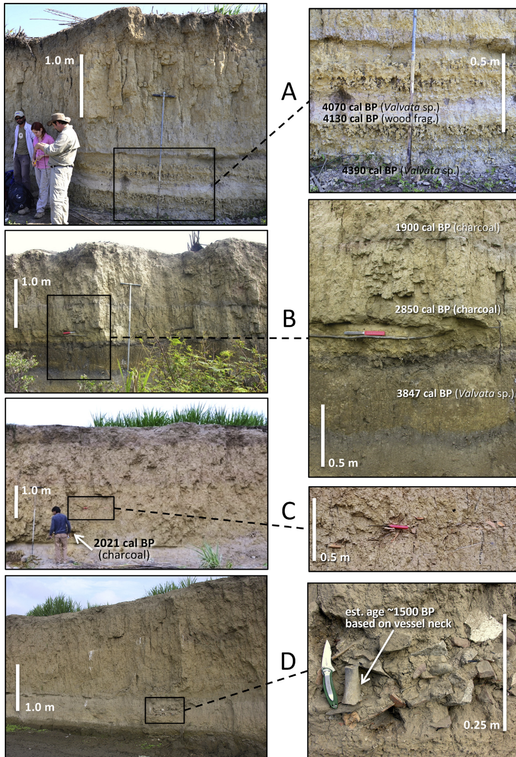
Fig. 6. Field photos showing thick floodplain deposits that have aggraded in the last few thousand years. Image sets A and B are from two locations near the coast and show a transition in soils after ~3.5 ka from slowly accreting calcic gleysols to rapidly accreting mix of natural cambic fluvisols and anthrosols. Image sets C and D are from the middle valley near Roma, ~30 km inland. These sites also show thick, rapidly aggrading floodplain deposits after ~2.0 ka due to increased ENSO-driven river discharge and irrigation diversions. Radiocarbon ages from Goodbred et al. (2017).
