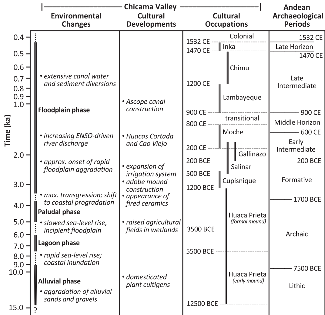
Fig. 3. Regional timeline showing the lower Chicama River valley's major environmental phases, cultural developments, and occupations alongside of the principle Andean archaeological periods. Note log-scale for time.
