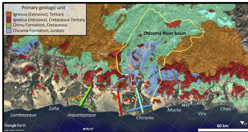
Fig. 2. Northern Peru coast and Andes mountains showing major geological formations (after Institute of Geology and Minerals, 1975) and mouths of the principal river valleys (image: Landsat; Google Earth). Note that the Chicama River basin (outlined in yellow) drains the region's largest exposure of the Chicama and Chicma Formations. The Chicama Formation is composed of metamorphosed mudstones and pelites that yield a relatively high fraction of fine-grained sediment. Also shown are the locations of the topographic profiles in Fig. 4 (green, red, and blue lines). (For interpretation of the references to color in this figure legend, the reader is referred to the Web version of this article.)
