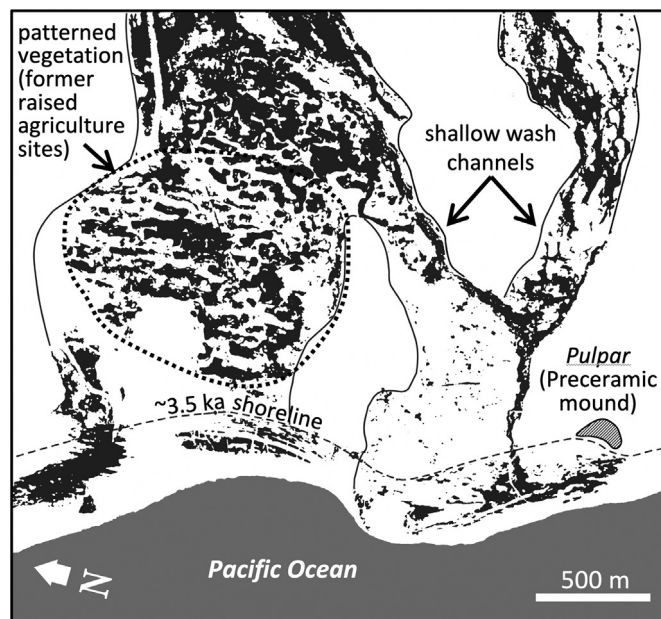
Fig. 5. Rendered image of ephemeral wash channels and raised-agricultural fields from the northern Chicama River valley. The black areas on the image denote vegetation, and location of the image is shown in Fig. 1. These wash channels are only active during the largest flood events and are typically scoured 1–3 m below the adjacent gravelly fan surface. This scour places the channel base closer to the water table, supporting the growth of thick vegetation during the long periods between major floods (decades to centuries). The particular location shown here hosts a large area (~1 km 2 ) of patterned vegetation that reflects its prior use in raised-field agriculture (camellones), which would have been active when this site comprised wetlands and ephemeral open-water habitat (see Fig. S5, for example). These agricultural plots also lie adjacent to a Preceramic mound, Pulpar, that is roughly contemporaneous with early Formative phase of Huaca Prieta (Dillehay, 2017).
