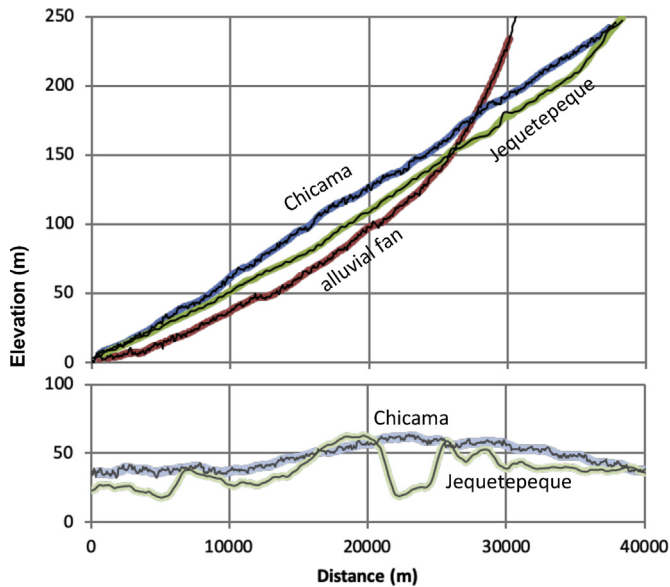
Fig. 4. Along-valley topographic profiles (upper panel) of the Chicama and Jequetepeque river fans, and an intervening alluvial fan system. Note the higher elevation and persistent slope of the aggrading Chicama and Jequetepeque valleys compared with the lower, concave profile of the alluvial fan surface. Cross-valley topographic profiles (lower panel) show broadly convex profiles of the two river fans, but the Jequetepeque River is > 30 m incised in its valley and thus decoupled from its adjacent fan surface. The Chicama River is not incised and can actively disperse sediment to its fan surface during overbank flooding. Profile locations are shown in Fig. 2.
