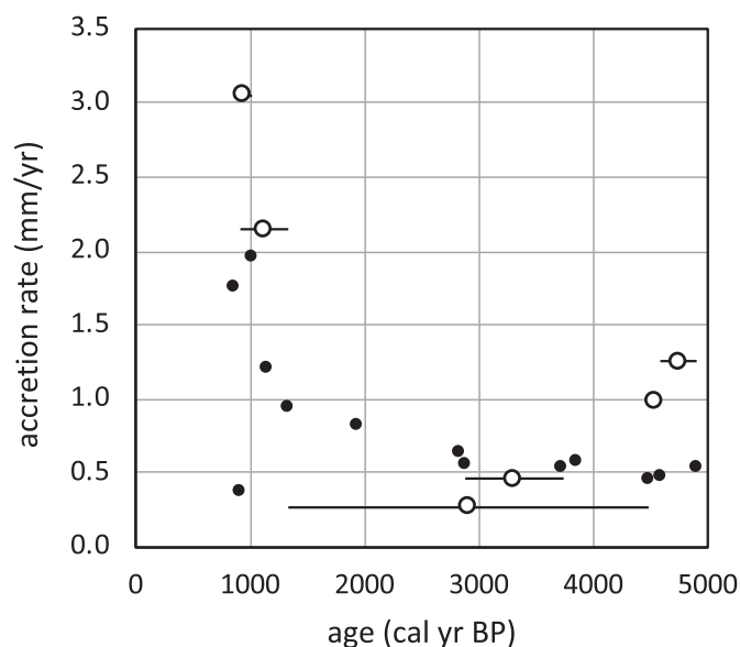
Fig. 7. Plot of long-term floodplain accretion rates over the mid-late Holocene period. Rates are interpolated from radiocarbon ages (Goodbred et al., 2017). Note that accretion rates increase significantly in the last 2000 years in association with more persistent ENSO-driven river discharge and the expansion of irrigation canals diverting sediment to the distal floodplain. Open circles represent rates interpolated between ages as shown by error bars; filled circles are averaged from sample age to present. Note that similar rates between the discrete-period values (open circles) and inclusive-period values (solid circles) indicate that the Sadler effect is not a significant factor in these data (Sadler, 1981).
