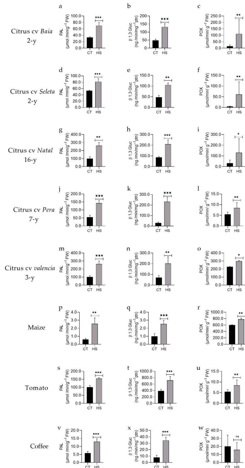
Figure 2. Enzymatic activity of phenylalanine ammonia-lyase (PAL), \beta -1,3-glucanase (GLUC), and peroxidase (POX) in different crops. Bars represent mean values from independent experiments with citrus cv. Baía (a–c), cv. Seleta (d–f), cv. Natal (g–i), cv. Pera (j–l), cv. Valencia (m–o), maize (p–r), tomato (s–u), and Coffea arabica (v–x). The enzymes assessed in each crop were PAL (first column), GLUC (second column), and POX (third column). Data were analyzed using Student's t -test. Asterisks indicate statistically significant differences compared to the control: p < 0.05 (*), p < 0.01 (**), p < 0.001 (***). "ns" indicates no statistically significant difference ( p > 0.05 ).
