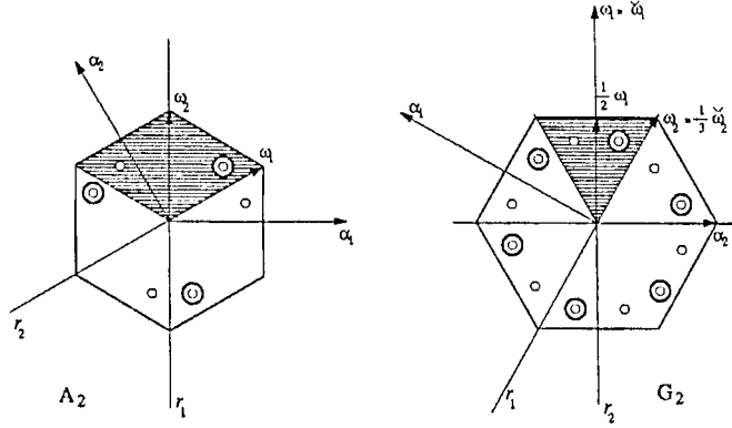
FIGURE 3. The simple roots, the fundamental weights, along with their dual, \tau_1, \tau_2 generators of W and the even fundamental region (shaded area) for A_2 and G_2 . The dots \circ denote the points of W -orbit and \bigcirc the points of W_e -orbit.
