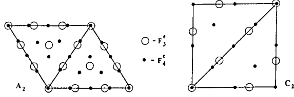
FIGURE 6. The lattice points of F_3^e, F_4^e in the fundamental region F^e for C_2 and A_2 .
