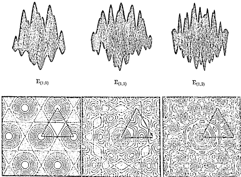
FIGURE 5. The E-functions for G_2 .
