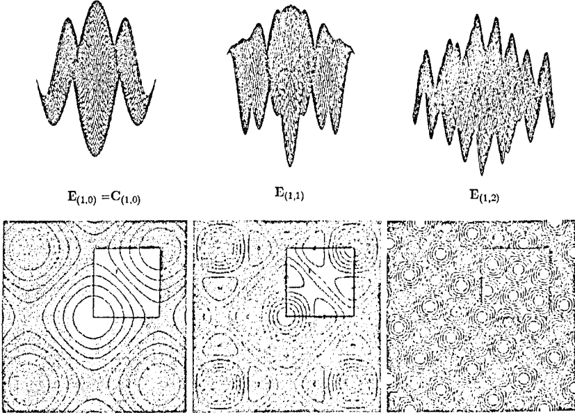
FIGURE 2. Examples of E-functions for C_2 .
