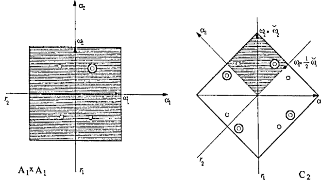
FIGURE 1. The simple roots, the fundamental weights, along with their dual, r_1, r_2 generators of W and the even fundamental region (shaded area) for A_1 \times A_1 and C_2 . The dots \circ denote the points of W -orbit and dots \bigcirc denote the points of W_e -orbit.
