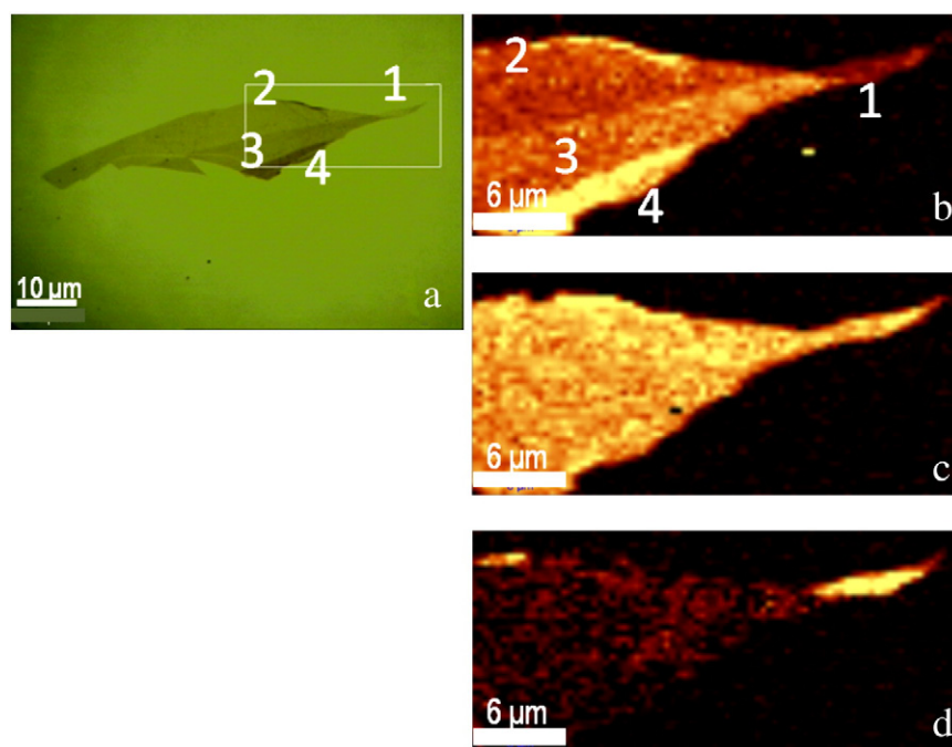
Fig. 1. Optical image of single (1), bi (2), few layers (3) and many layers (4) regions of graphene on \text{SiO}_2/\text{Si} substrate, for the sample m4, before deposition of Au-NPs (a). Raman images mapped with the integrated intensities of the G band ( 1580\text{ cm}^{-1} ) (b) and 2D bands at 2690\text{ cm}^{-1} (c) and 2671\text{ cm}^{-1} (d) after deposition of Au-NPs.
