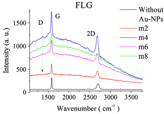
Fig. 4. Comparison of the Raman intensities of FLG before (black curve) and after deposition of Au-NPs (same colours as in Fig. 3, 1 = without Au-NPs, 2 = m2, 3 = m4, 4 = m6, 5 = m8).
