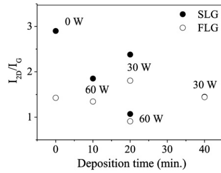
Fig. 5. Integrated intensity ratio between the 2D band and G band ( I_{2D}/I_G ) of SLG (black dots) and FLG (empty dots) before (without Au-NPs) and after deposition of Au-NPs at the two DC powers and deposition times. As the time increases the ratio for SLG and FLG remains practically the same (30 W/40 min.).
