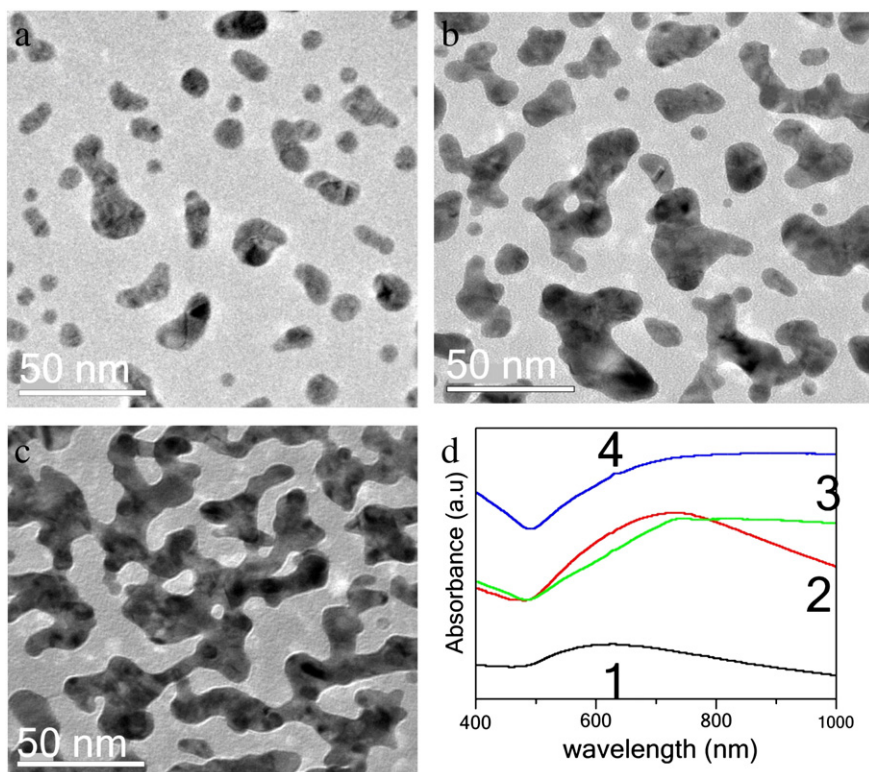
Fig. 2. TEM images of Au-NPs. a) 30 W/20 min, b) 30 W/40 min, c) 60 W/10 min and d) UV–vis spectra of the Au-NPs, shown in Fig. (a–c), 30 W/20 min (1, black), 30 W/40 min (2, red), 60 W/10 min (3, green) and 60 W/20 min (4, blue).
