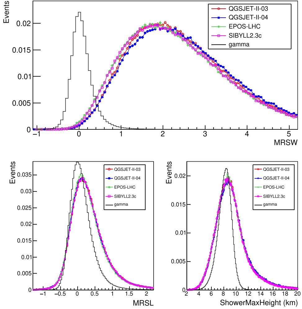
Figure 6. Distributions of basic shower parameters for proton events produced with the four interaction models, for energies E_{\text{rec},\gamma} of 1–10 TeV. Histograms are normalized by areas (number of the accepted events). The difference in shower rates from the effect shown in figure 4 is not included. (Top) MRSW, (bottom left) MRSL, (bottom right) height of shower maximum, measured from the observation level.
