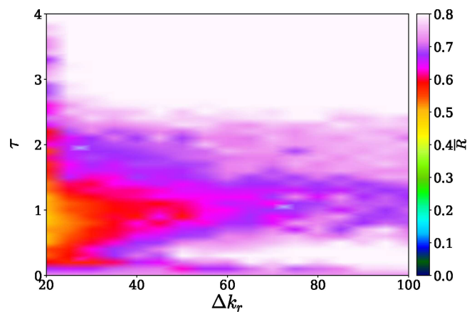
FIG. 8. Averaged order parameter of the whole brain network under a random pulsed current as a function of \tau and \Delta k_r for \nu_0 = 8 , e = 0.1 , and c = 0.05 .
