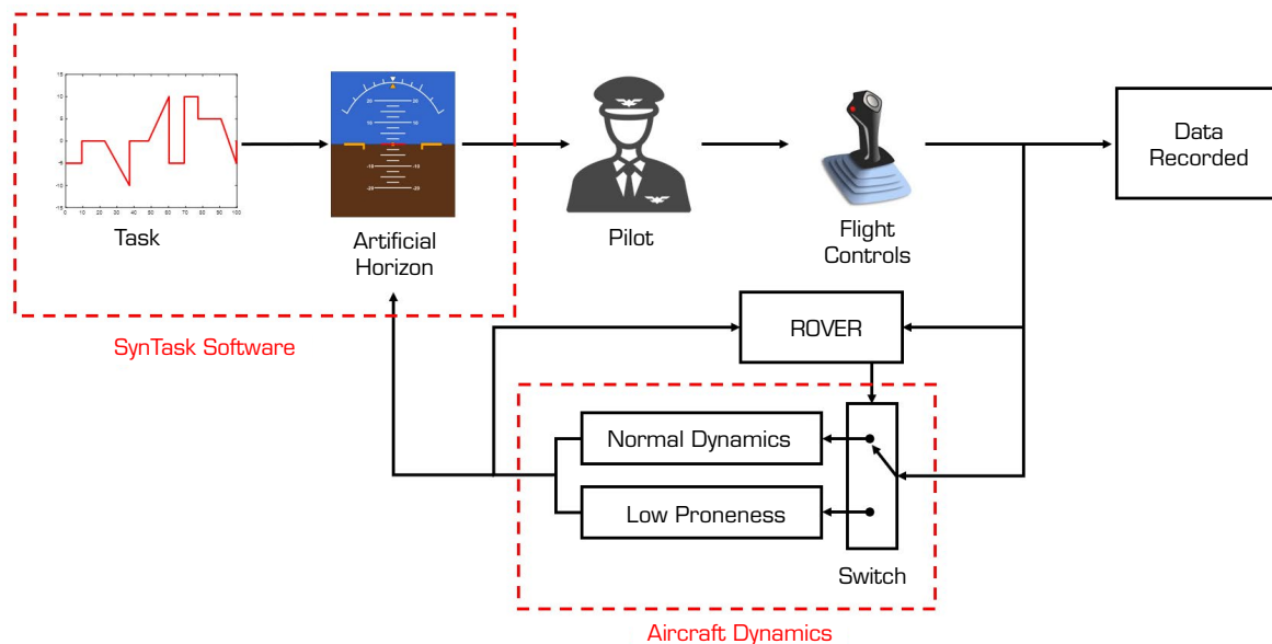
Figure 2. Suppression control system architecture.
