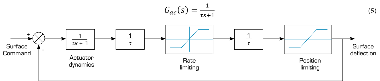
Figure 1. Aircraft surface actuator model.
