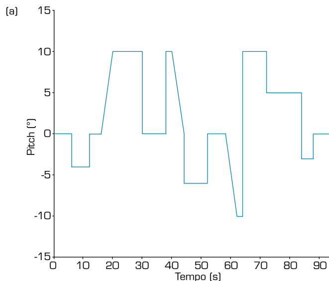
Figure 5. Task used during tests (a) and test bench (b).
