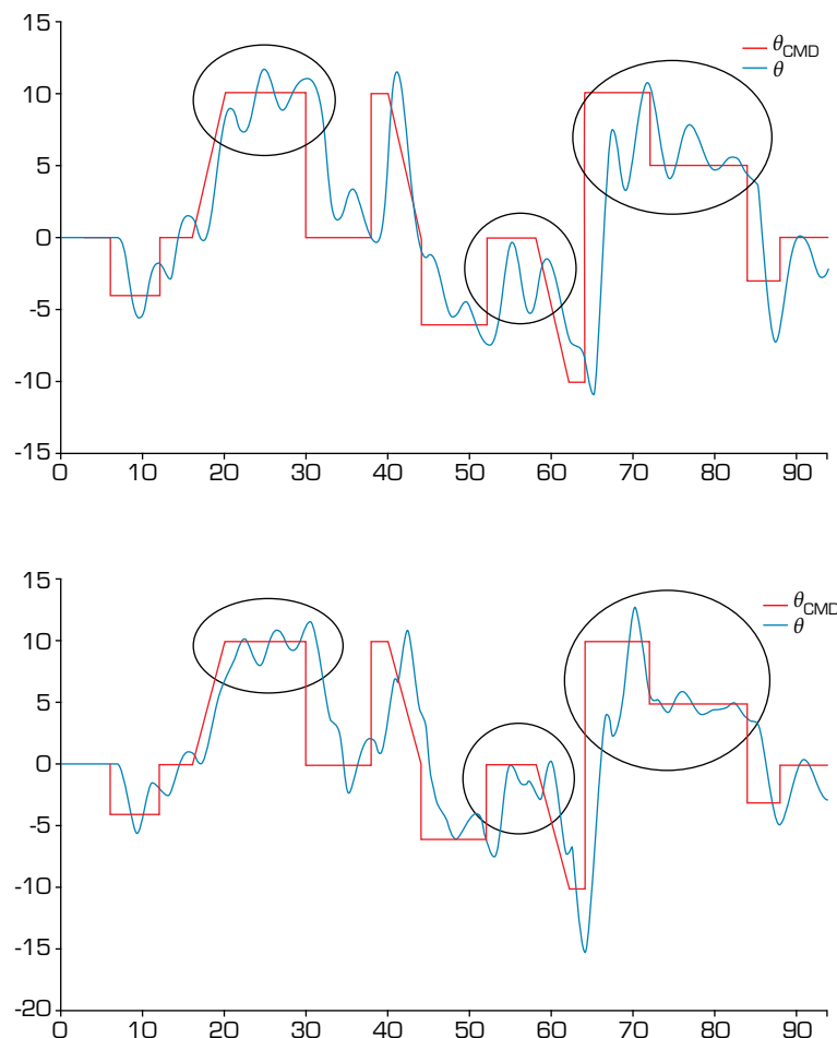
Figure 6. Temporal data from one of the volunteers without (a) and with (b) the suppression system.
