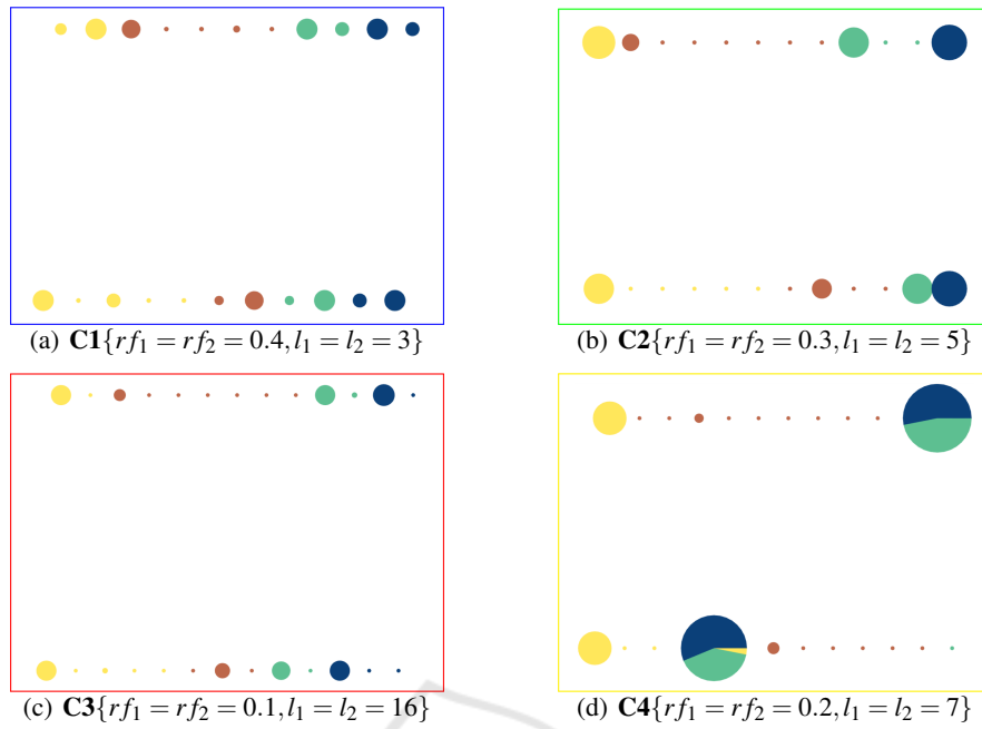
Figure 5: Coarsest graphs of the multilevel hierarchies computed for SG_1 with 4 distinct parameter settings in Gmb .
