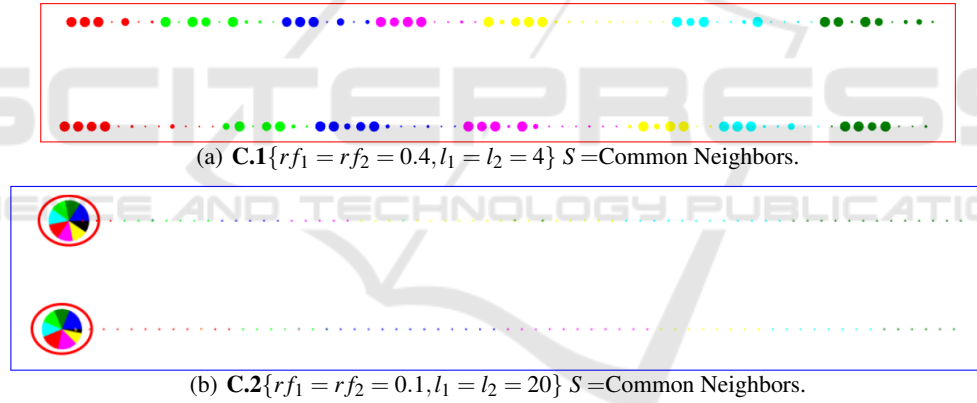
Figure 6: Coarsest graphs of the multilevel hierarchy obtained from graph SG_2 with two settings of Gmb .
