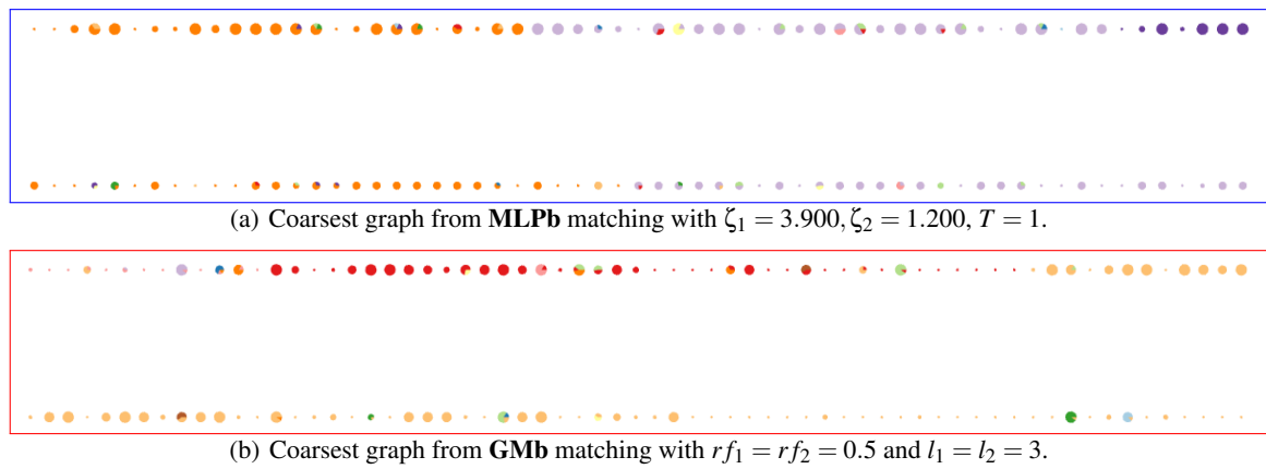
Figure 7: Coarsest level graphs after coarsening SG_5 with different matching algorithms and S=\text{Common Neighbors.}
