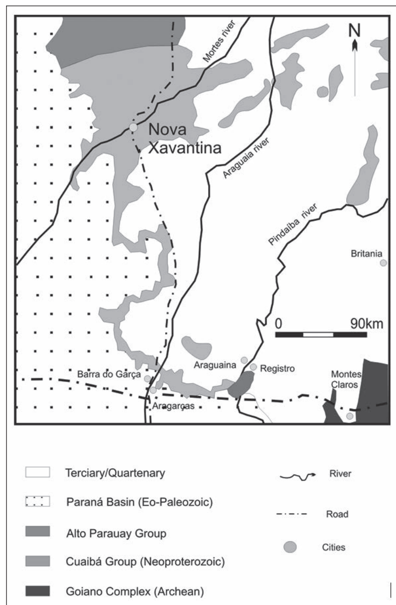
Figure 2 Regional geologic map of Nova Xavantina Region modified from Martinelli (1998). The Paraguay Belt (Cuiaba Group) rocks are partially covered: Cenozoic sediments (East), Paleozoic Paraná Basin rocks (West) and Alto Paraguay undeformed sedimentary rocks (North).
