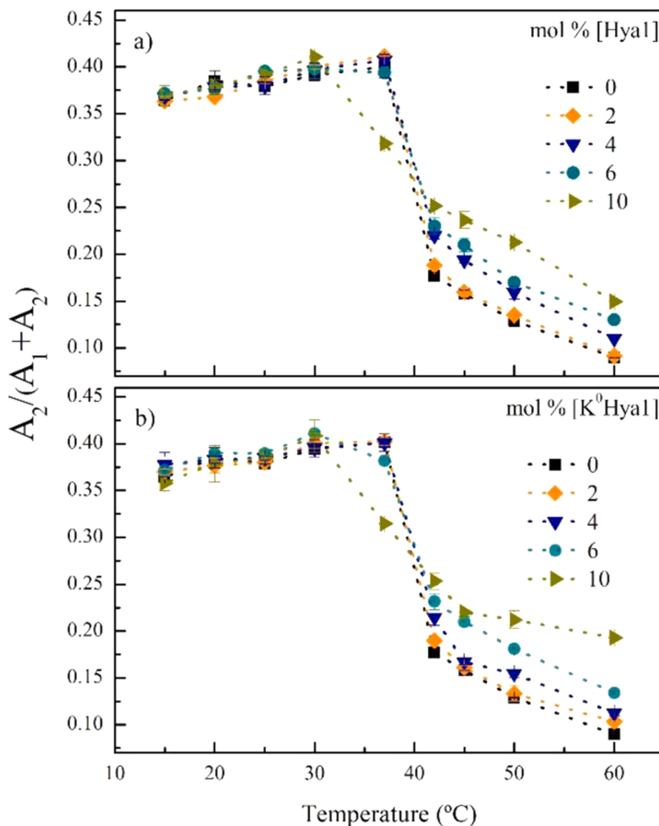
Fig. 5. The fraction of the area of the higher energy emission band ( A_2/(A_1 + A_2) ) as a function of the temperature for pure DPPG (black squares), and in the presence of Hya1 (Fig. 5a) or K 0 Hya1 (Fig. 5b). Relative percentage of the peptides are: 2 mol% (orange diamonds), 4 mol% (blue down triangles), 6 mol% (dark cyan circles), and 10 mol% (dark yellow right triangles). (For interpretation of the references to colour in this figure legend, the reader is referred to the web version of this article.)
