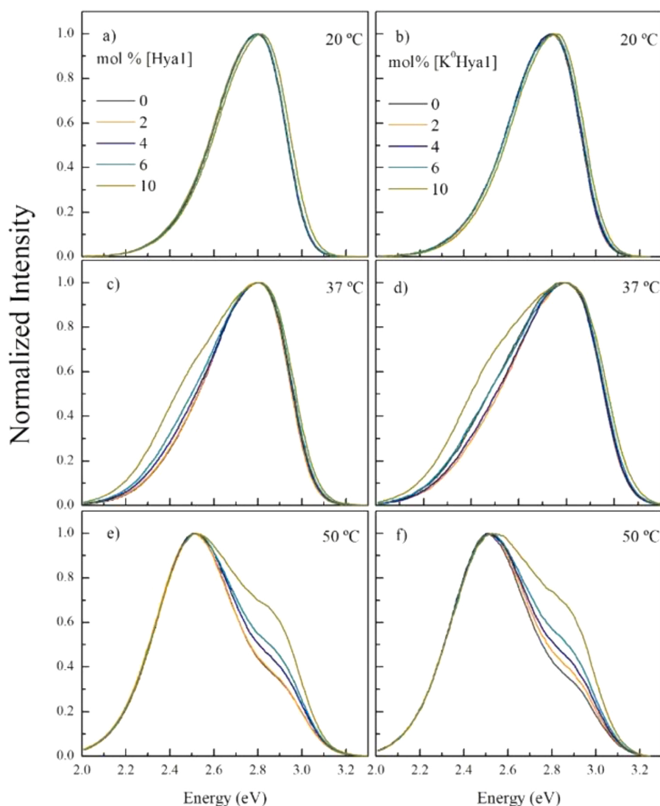
Fig. 4. Emission spectra of Laurdan ( 5 \mu\text{mol L}^{-1} ) incorporated into DPPG ( 500 \mu\text{mol L}^{-1} ) vesicles in the absence and with different concentrations of HyaI (left column) or \text{K}^0\text{HyaI} (right column), at three temperatures, 20 °C (a,b), 37 °C (c,d), and 50 °C (e,f). Peptide/lipid concentrations: 0 (black lines), 2 mol% (orange lines), 4 mol% (blue lines), 6 mol% (dark cyan lines), and 10 mol% (dark yellow lines). (For interpretation of the references to colour in this figure legend, the reader is referred to the web version of this article.)
