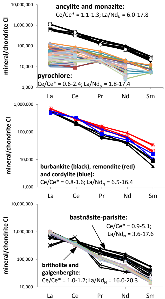
Fig. 11. LREE patterns of REE-bearing minerals normalized to chondrite CI (Barrat et al., 2012); Ce/Ce^* = Ce/(La \cdot Pr)^{0.5} , La/Nd_N = La/Nd (both normalized to chondrite CI).
