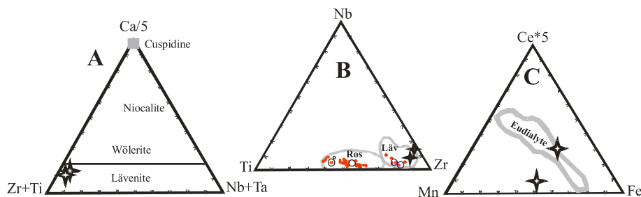
Fig. 10. A: Ca/(Nb + Ta)–(Zr + Ti) ternary diagram with data points corresponding to the lăvenite analyses of Table 9 (stars) and the main composition of the cuspidine group (grey full square), after Keller and Williams (1995). B: Nb–Ti–Zr cation distribution (after Keller and Williams, 1995), for rosenbuschite (Ros) and Lăvenite (Lăv). Large circles: rosenbuschite and lăvenite from Table 9; stars, eudialyte. Red dots: compositions from Carbonin et al. (2005). C: Fe–Mn–Ce*5 ternary diagram for eudialytes (field of eudialyte from Sjöqvist et al., 2013).
