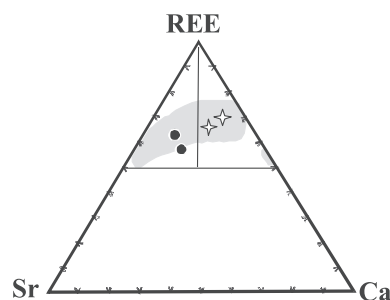
Fig. 9. REE-Sr-Ca variation diagram for ancylite (full circles) and galgenbergite (stars) from Cerro Boggiani samples (cf. Table 7). The grey field represents the composition of world-wide ancylites and Ca-ancylites after Pekov et al. (1997).
