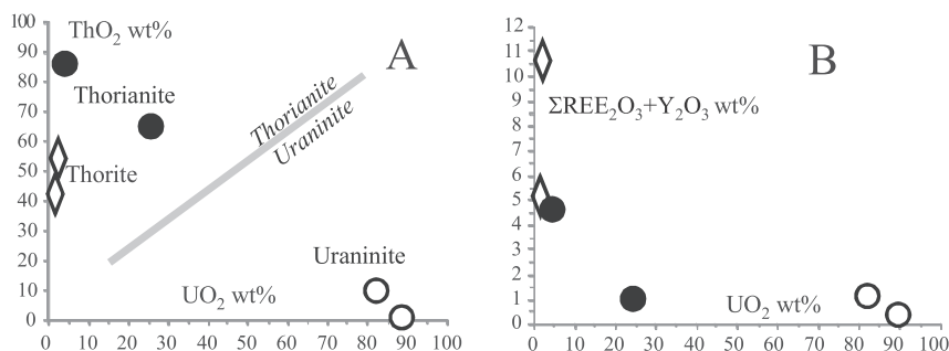
Fig. 6. UO 2 vs. ThO 2 (A) and UO 2 vs. ΣREE + Y 2 O 3 (B) of thorianite, uraninite and thorite crystals from the Cerro Boggiani complex (after Förster, 1999 and references therein).
