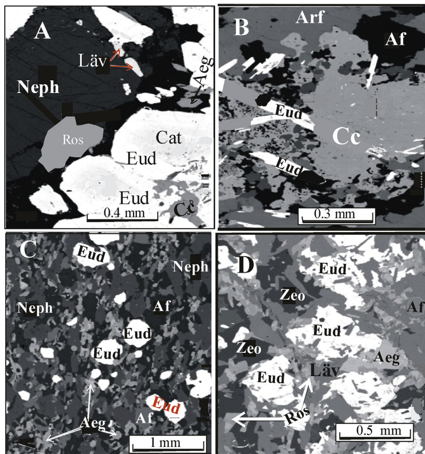
Fig. 2. Back-scattered Scanning Electron Microscope (SEM) images of fundamental and accessory minerals from the Cerro Boggiani agpaite alkaline igneous rocks. A: large eudialyte (Eud) from nepheline syenite (RP33B) with catapleiite (Cat), nepheline (Neph), calcite (Cc), rosenbuschite (Ros) and lävenite (Läv); B: nepheline syenite (RP33B) showing eudialyte (Eud), arfvedsonite (Arf), calcite (Cc) and alkali feldspar (Af); C: fine grained eudialyte (Eud) in phonolitic lava flow (RP31A) associated with nepheline (Neph), alkali feldspar (Af) and aegirine (Aeg); D: eudialyte in nepheline syenite (RP33B), with zeolites (Zeo), aegirine (Aeg), alkali feldspar (Af) and rosenbuschite (Ros).
