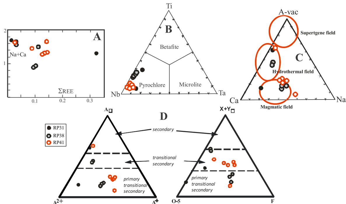
Fig. 7. A: Na + Ca (a.f.u.) vs. REE for pyrochlore samples. B: Ti–Nb–Ta pyrochlore compositional diagram (cf. Hogarth and Horne, 1989 and references therein). C: Ca–Na–A vacancies plot showing representative compositions of pyrochlore from Cerro Boggiani. The fields are after Zurevinski and Mitchell (2004 and references therein). D: Triangular plots showing the atomic percentage variations of A-site vacancies ( A Y), X + Y anion vacancies ( X+Y Y), divalent and monovalent A-site cations (A 2+ and A + ), oxygen (plotted as O-5) and fluorine (F) in the Cerro Boggiani pyrochlores. The maximum amount of vacancies due to primary (T ca. 300–550 °C), transitional (T ca. 200–300 °C) and secondary (T < 150 °C) alterations are also reported; after Lumpkin and Ewing (1995).
