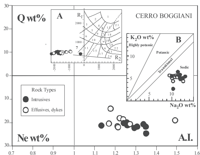
Fig. 3. Cerro Boggiani complex (data from Comin-Chiaramonti et al., 2005): agpaite index [A.I. = (\text{Na}_2\text{O} + \text{K}_2\text{O})/\text{Al}_2\text{O}_3 , molar ratio] vs. normative quartz (Q) and nepheline (Ne) for sodic rock-types. Inset A: R_1 – R_2 classification diagram according to De La Roche et al. (1980) showing field 7, i.e. nepheline syenite-phonolite. Inset B: \text{Na}_2\text{O} vs. \text{K}_2\text{O} wt% diagram (after Le Maitre, 1989) displaying the sodic field occupied by the Cerro Boggiani samples.
