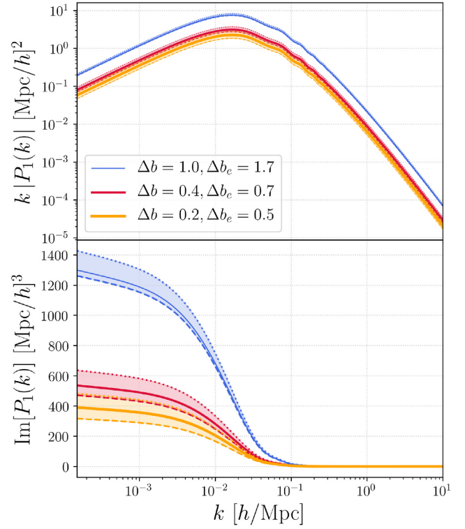
Figure 1. Theoretical prediction for the cross power spectrum dipole of different tracers at redshift z = 1.9 , with the difference in linear and evolution bias shown in the legend. Solid lines represent the case where there is no magnification bias s_\alpha = 0 , whereas shaded regions represent the effect of different magnification biases among the tracers. Dotted lines show the limiting case where s_\alpha is smaller than s_\beta by 40 per cent, whilst the dashed ones show the opposite case, with s_\alpha larger than s_\beta by a factor of 40 per cent.
