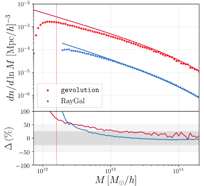
Figure A1. Comparison between the halo mass function of the catalogue employed in this analysis (stars), with the one from the full-sky RayGal simulation (dots) from Breton et al. (2018), with both catalogues in real space. Solid curves correspond to the Tinker mass function fit (Tinker et al. 2008), while the bottom panel shows the relative difference between the fit prediction and the mass function computed from the simulations. Vertical dashed line corresponds to the limit of gevolution haloes with at least 600 particles. The cosmological parameters in the RayGal simulation that differ from ours are h = 0.72 , A_s = 2.431 \times 10^{-9} , \Omega_m = 0.257 , T_{\text{cmb}} = 2.726 . We stress that the RayGal mass function was multiplied by a 0.1 factor for a cleaner visualization, as the values were very similar. Differences between the Tinker and Sheth–Tormen (Sheth & Tormen 1999) mass functions were minor, so we only present the former.
