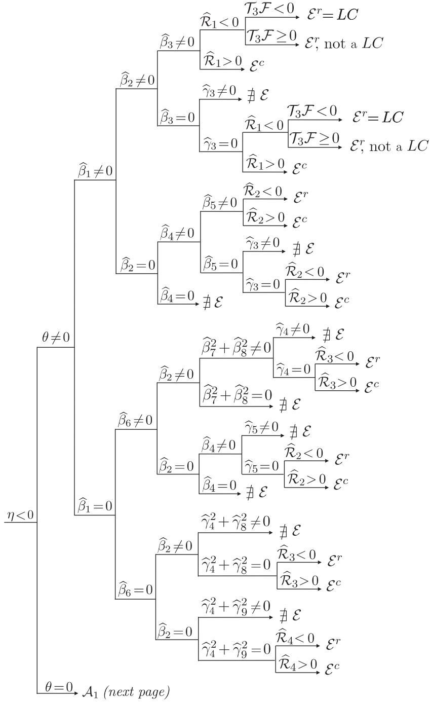
DIAGRAM 1: The existence of invariant ellipse: the case \eta < 0
