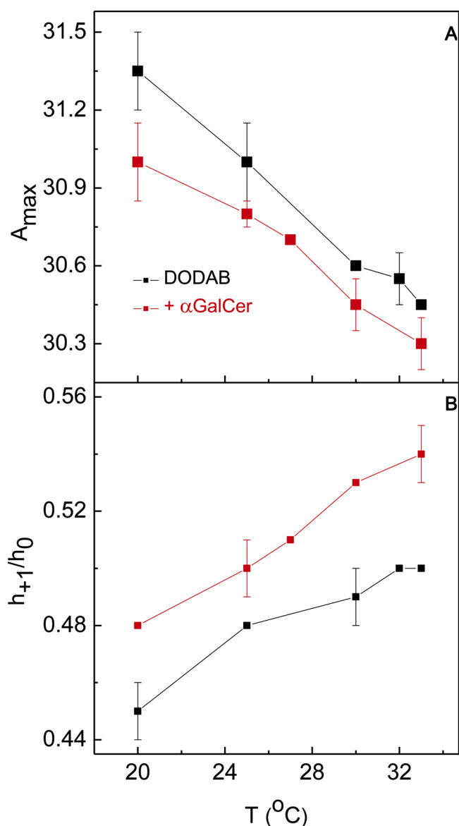
Fig. 4. Effect of 0.2 mM \alpha -GalCer on the maximum hyperfine splitting ( A_{max} ) of 5-PCSL (A) and on the ratio of the low and the central field line amplitudes ( h_{+1}/h_0 ) of 16-PCSL (B) embedded in 2 mM DODAB bilayers at the gel phase. Error bars indicate standard deviations of at least two experiments with different samples.
