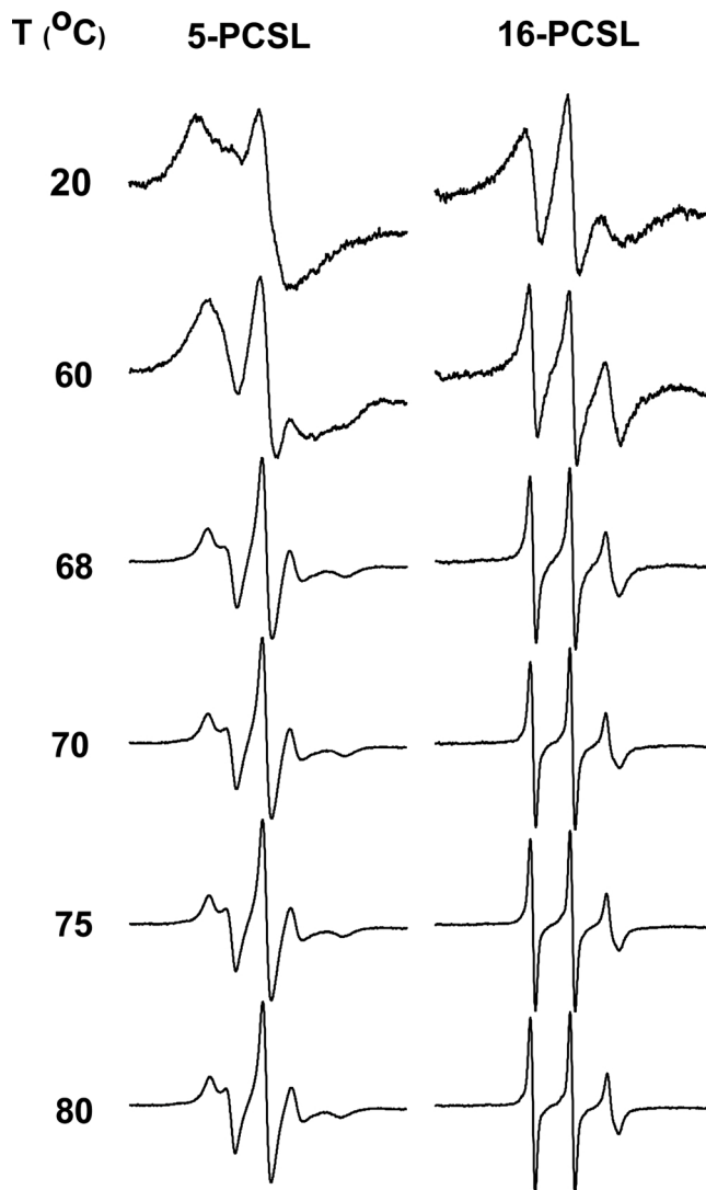
Fig. 7. Effect of temperature on the ESR spectra of 5-PCSL and 16-PCSL embedded in assemblies of 2 mM \alpha -GalCer. Total spectra width is 100 G.
