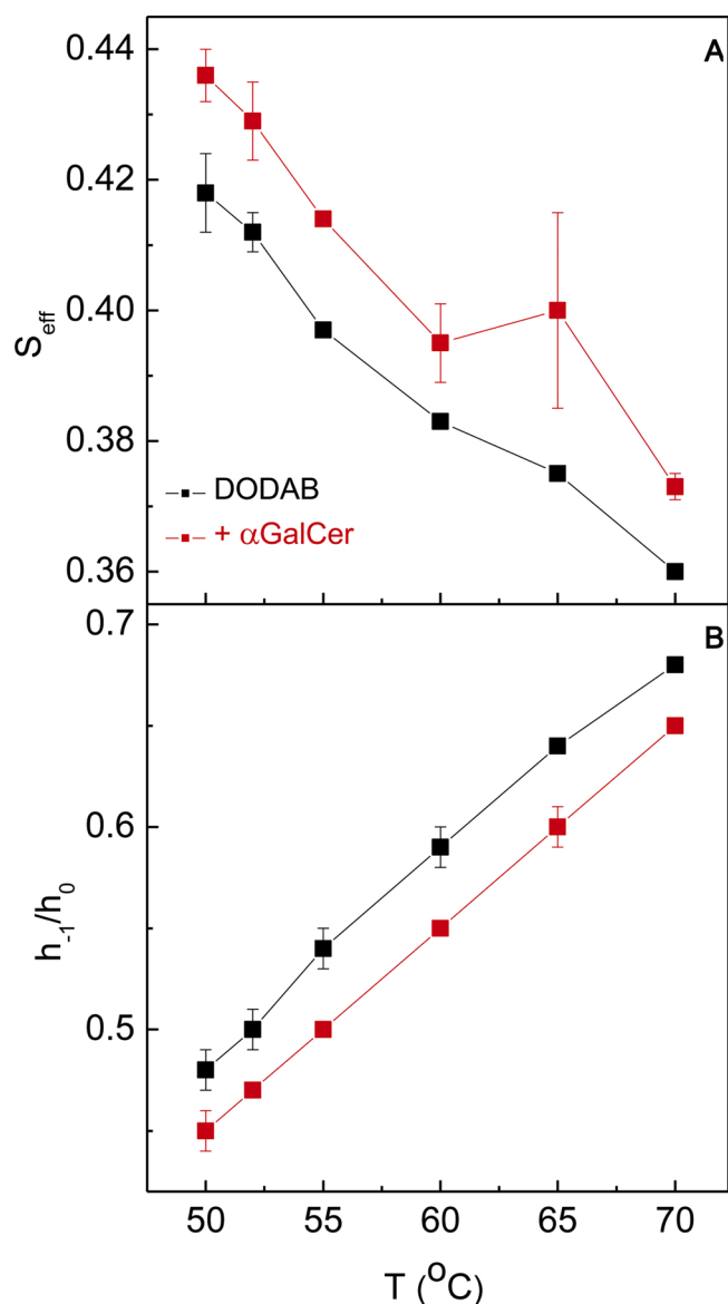
Fig. 6. Effect of 0.2 mM \alpha -GalCer on the effective order parameter ( S_{eff} ) of 5-PCSL (A) and on the h_{-1}/h_0 ratios of 16-PCSL (B) embedded in 2 mM DODAB bilayers at the fluid phase. Error bars indicate standard deviations of at least two experiments with different samples.
