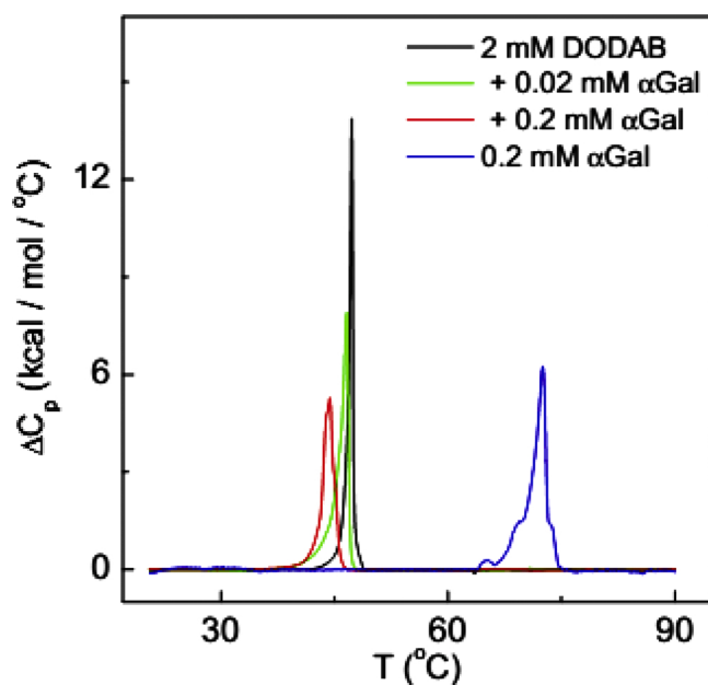
Fig. 2. Effect of \alpha -GalCer on the DSC thermogram of 2 mM DODAB bilayers. Scan rate was 20 °C/h.
