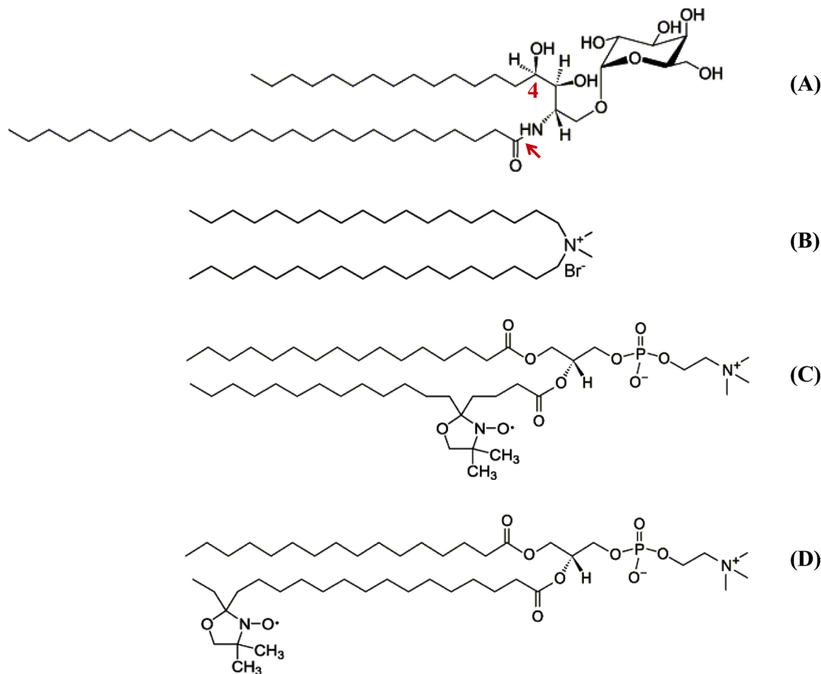
Fig. 1. Chemical structures of \alpha -GalCer (A), DODAB (B), 5-PCSL (C) and 16-PCSL (D). In (A), the arrow indicates the amide bond connecting the acyl chain to the phytosphingosine and the number 4 indicates the hydroxyl group bonded to carbon 4 of the phytosphingosine.
