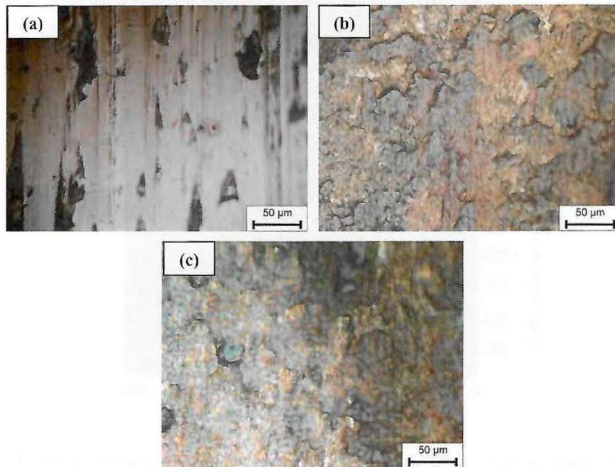
Figure 7. Aspects of the interiors of the adhesive wear caps. Distance traveled: 642.11 m (last run). (a) Ductile iron, (b) borided ductile cast iron and (c) ductile iron with thermally sprayed layer.
