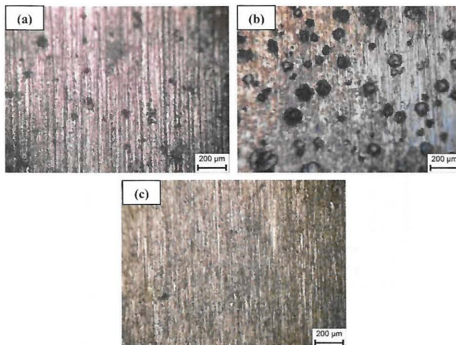
Figure 6. Aspect of the interior of the abrasive wear cap. Distance traveled: 481.58 m (last run). (a) Ductile iron, (b) borided ductile cast iron and (c) ductile iron with thermally sprayed layer.
