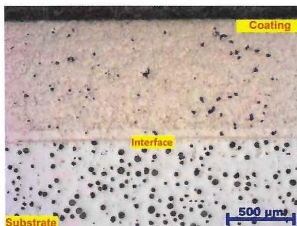
Figure 3. Nodular cast iron – Thermal sprayed NiCrBSi alloy. Coating melting temperature of 1000 ° C. Permanency time in the oven 20 minutes. No chemical etching.
