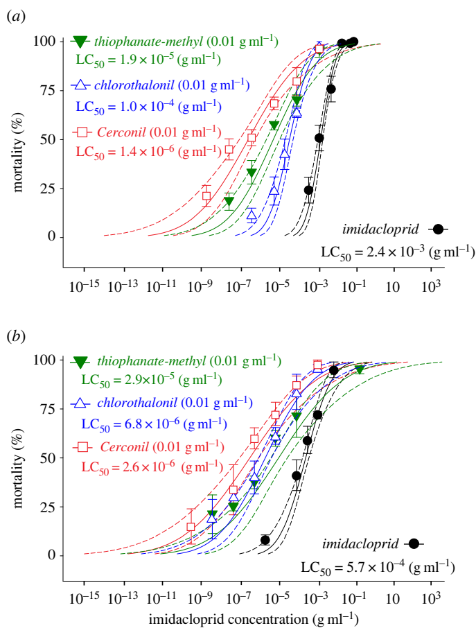
Figure 3. Effects of combined exposure to the neonicotinoid imidacloprid and fungicides on bee mortality. Concentration–mortality curves of Apis mellifera (a) and Partamona helleri (b) exposed to mixtures of imidacloprid and the fungicides chlorothalonil (ch), thiophanate-methyl (tm) and Cerconil (mixture of chlorothalonil and thiophanate-methyl). LC_{50} values are indicated and dotted lines represent the 95% fiducial limits of each curve. Symbols represent concentrations tested (on x-axis) and observed mortality (on y-axis). Vertical bars represent standard error (s.e.) of the mean.
